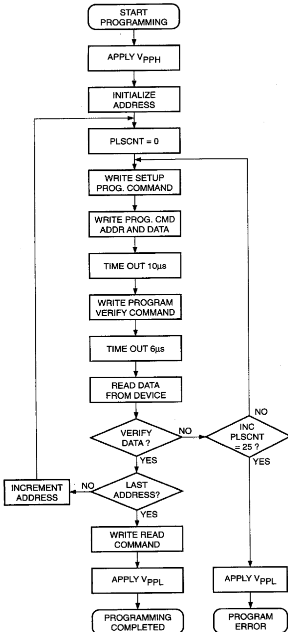
Figure 7. Programming Algorithm(1)
