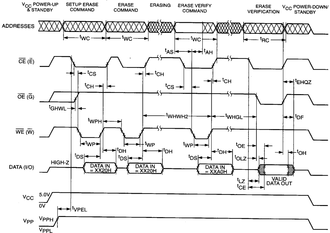
Figure 4. A.C. Timing for Erase Operation
