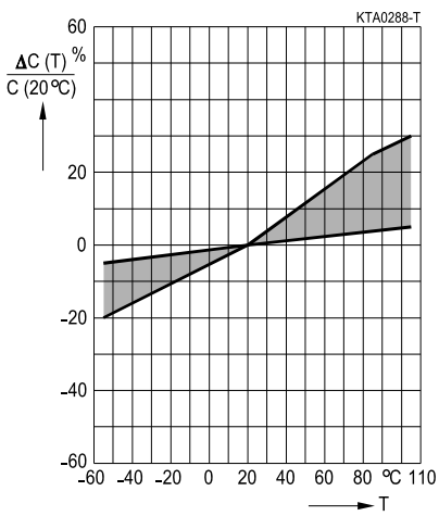
Capacitance change versus temperature (typ. values)
