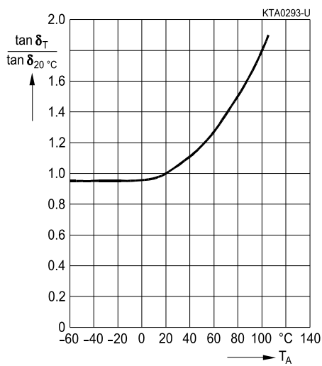
Dissipation factor versus temperature at f = 120 \text{ Hz}
