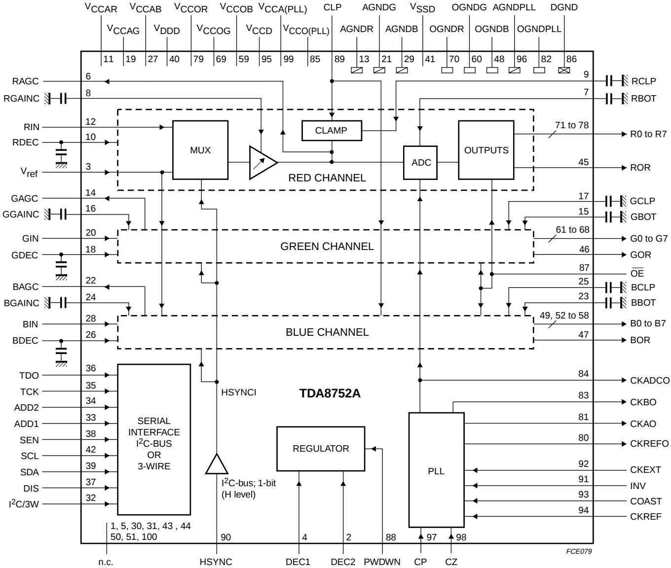
Fig.1 Block diagram.
