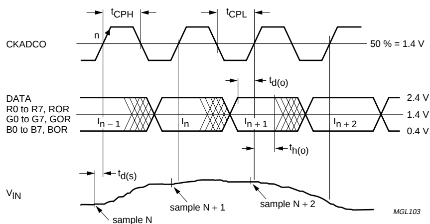
Fig.11 Timing diagram.
