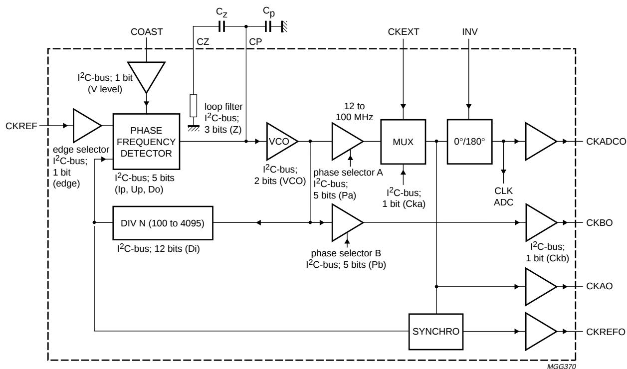
Fig.3 PLL diagram.
