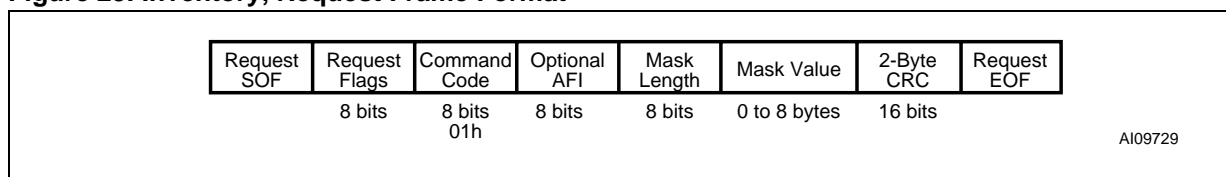
Figure 23. Inventory, Request Frame Format
