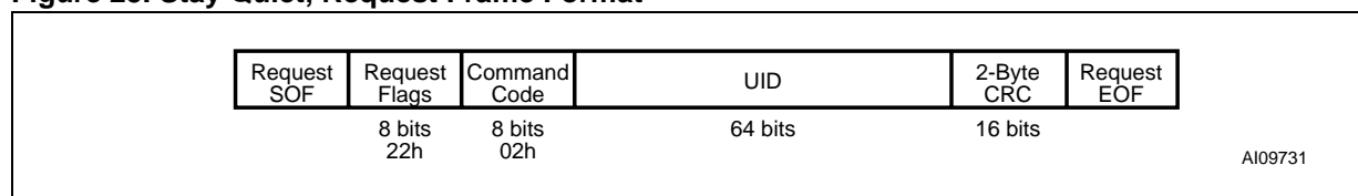
Figure 25. Stay Quiet, Request Frame Format
