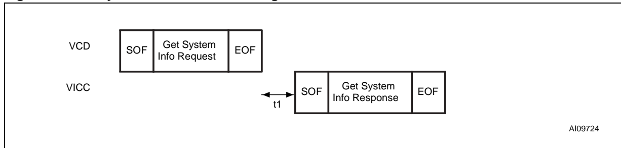
Figure 38. Get System Info Frame Exchange between VCD and LRI64
