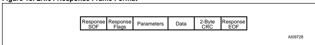
Figure 18. LRI64 Response Frame Format
