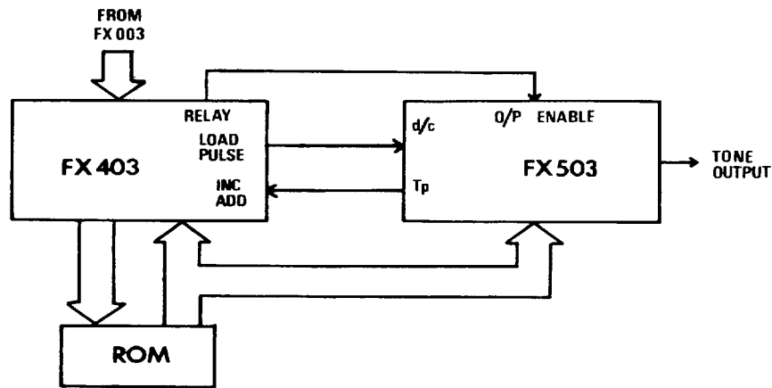
FIG. 5 TRANSPOND ARRANGEMENT
