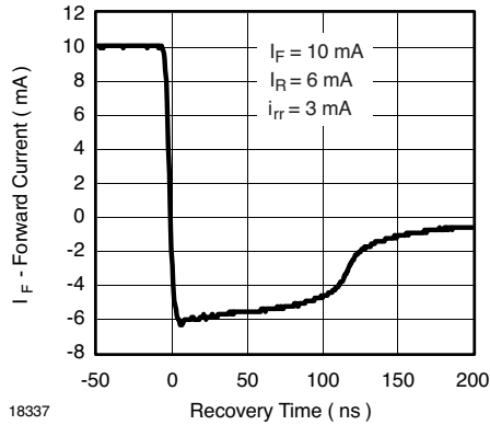
Fig. 5 Typical Charge Recovery Curve
