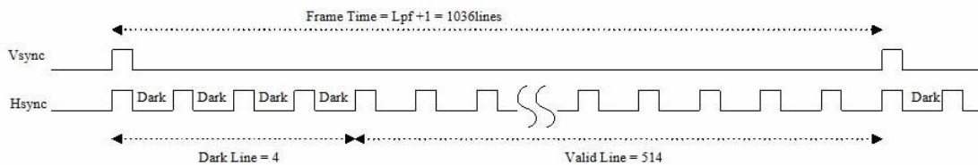
Figure 3.10 Inter-frame timing
