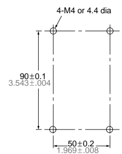
Mounting dimensions (Bottom view)
