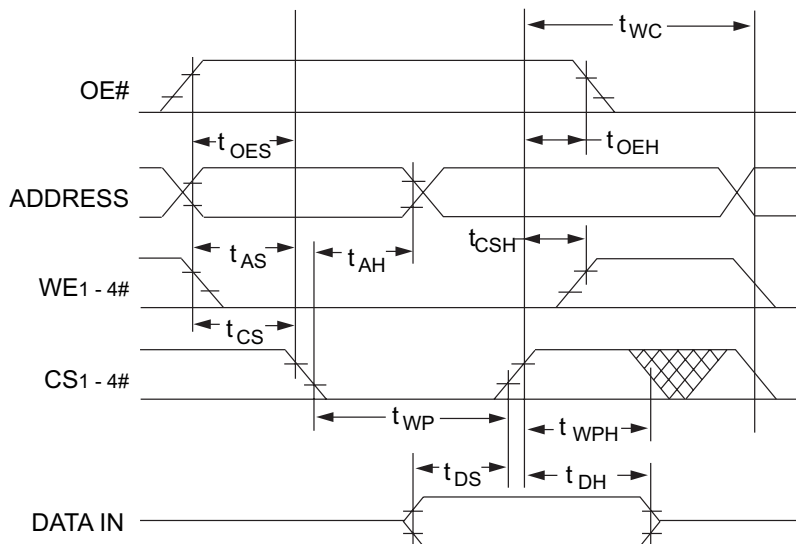
FIGURE 5 – WRITE WAVEFORMS CS# CONTROLLED
