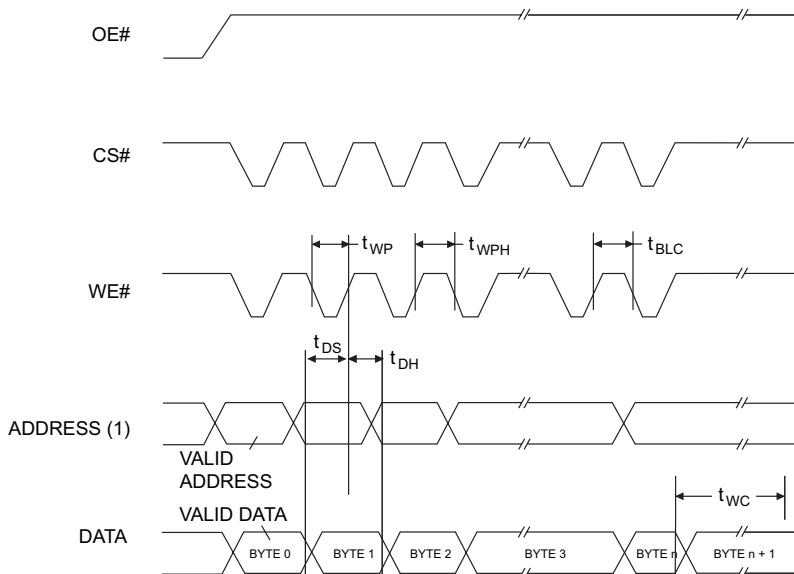
FIGURE 8 – PAGE WRITE WAVEFORMS
