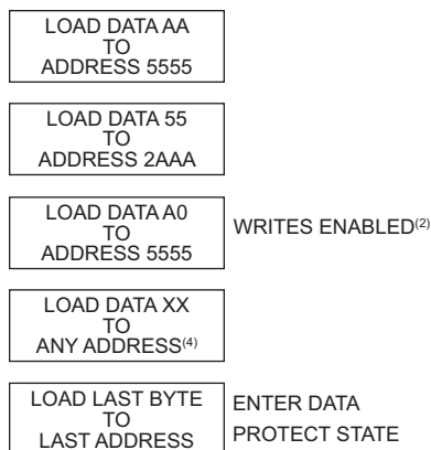
FIGURE 9 – SOFTWARE BLOCK DATA PROTECTION ENABLE ALGORITHM (1)
