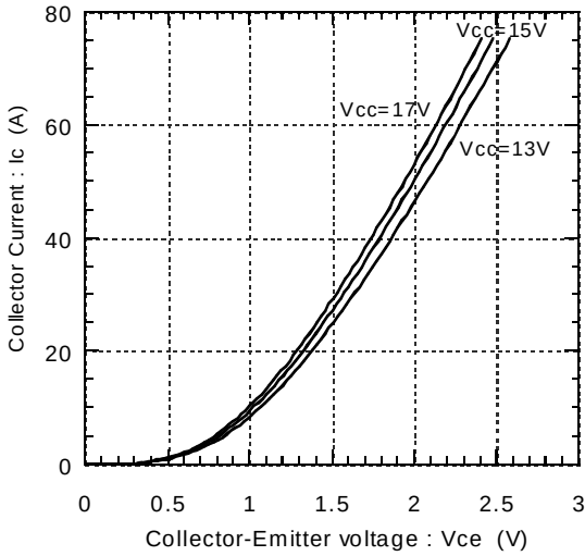
Collector current vs. Collector-Emittter voltage Tj=125°C
