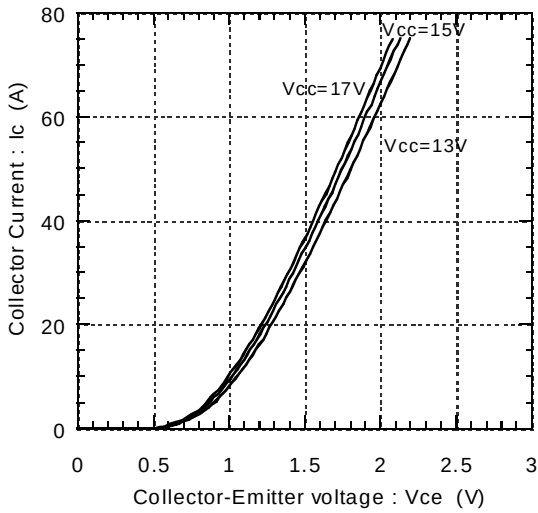
Collector current vs. Collector-Emittter voltage Tj=25°C
