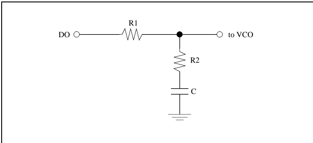
Fig. 3 – Passive low-pass filter circuit
