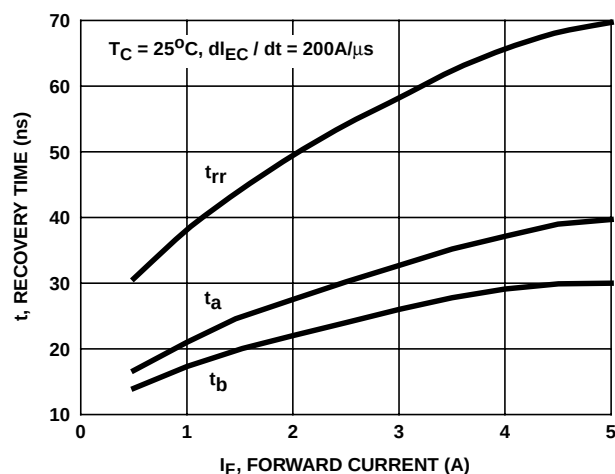
FIGURE 19. RECOVERY TIMES vs FORWARD CURRENT
