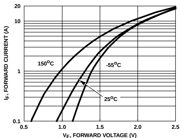
FIGURE 18. DIODE FORWARD CURRENT vs FORWARD VOLTAGE DROP
