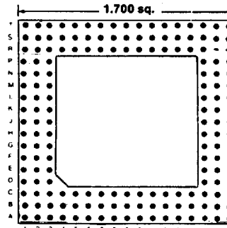
168 PINS Footprint 17009
