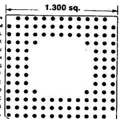
121 PINS Footprint 13058
