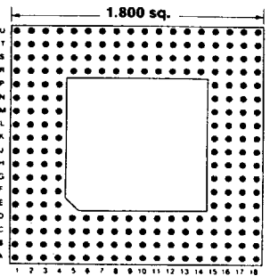
Footprint 18004
