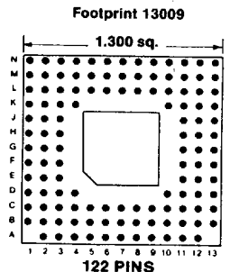
Footprint 13009
