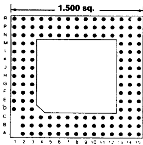
141 PINS Footprint 15028
