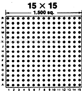
225 PINS Footprint 15001
