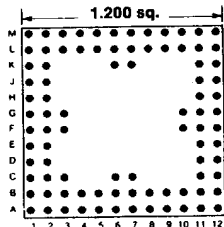
89 PINS Footprint 12007
