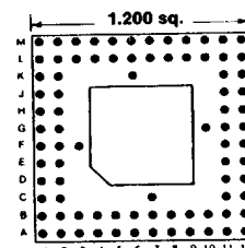
84 PINS Footprint 12010
