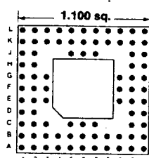
85 PINS Footprint 11007
