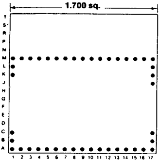
Footprint 17014
