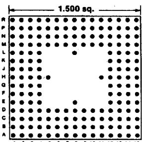
180 PINS Footprint 15008
