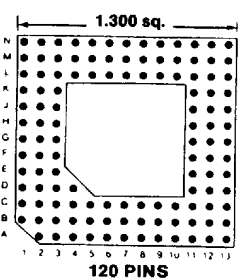
Footprint 13015
