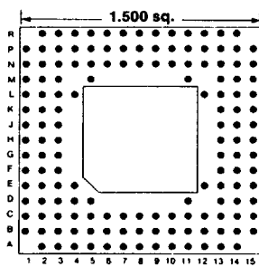
149 PINS Footprint 15018
