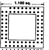
Footprint 11039
