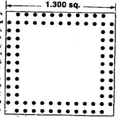
84 PINS Footprint 13053
