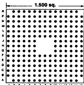
212 PINS Footprint 15004
