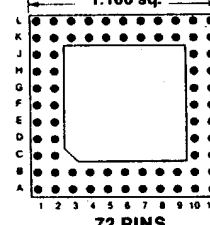
72 PINS Footprint 11023
