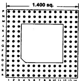
132 PINS Footprint 14015
