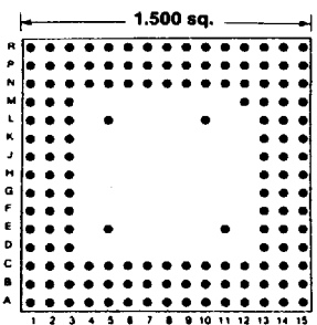
149 PINS Footprint 15020
