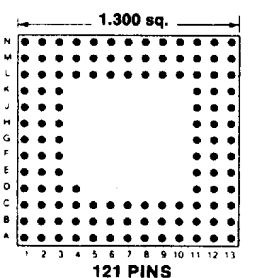
Footprint 13012
