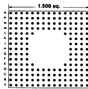
180 PINS Footprint 15010
