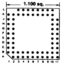
Footprint 11035
