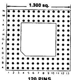
120 PINS
