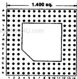
133 PINS Footprint 14013
