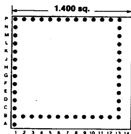
49 PINS Footprint 14020
