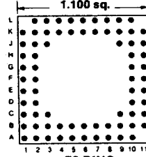
73 PINS Footprint 11022
