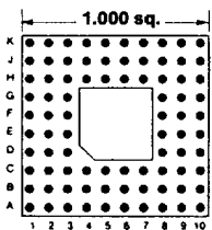
84 PINS Footprint 10002
