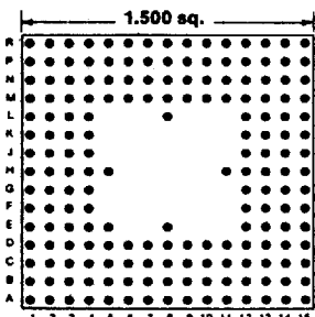
181 PINS Footprint 15006
