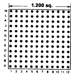
Footprint 12001
