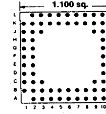
72 PINS Footprint 11025
