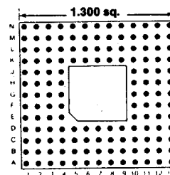
144 PINS Footprint 13002
