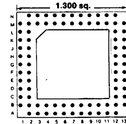
84 PINS
