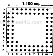
Footprint 11031
