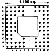
74 PINS Footprint 11017
