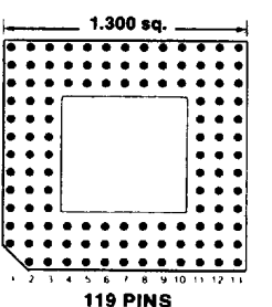
Footprint 13017
