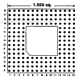
176 PINS Footprint 15013
