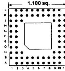
72 PINS Footprint 11026
