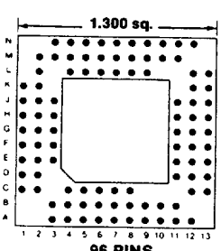
Footprint 13025
