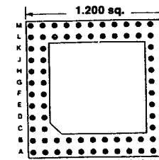
80 PINS Footprint 12014
