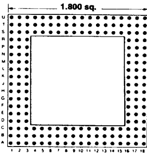
Footprint 18006
