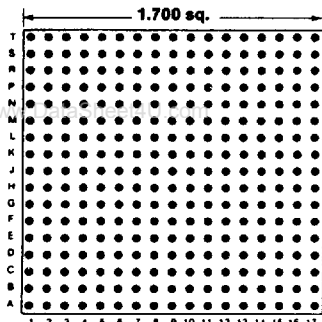
289 PINS Footprint 17001
