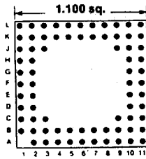
75 PINS Footprint 11016
