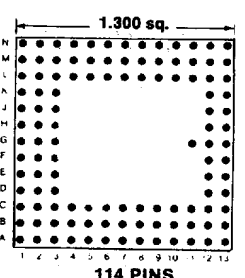
Footprint 13020
