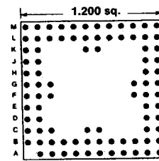
88 PINS Footprint 12009
