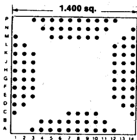
94 PINS Footprint 14022
