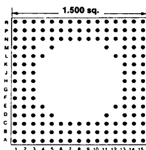
153 PINS Footprint 15017
