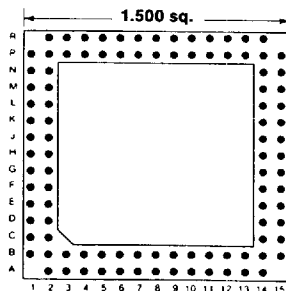
100 PINS Footprint 15030
