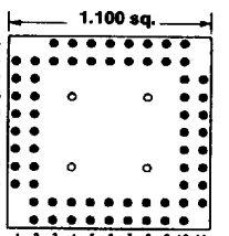
Footprint 11038
