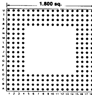
Footprint 18005
