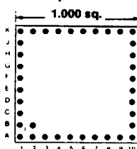
37 PINS Footprint 10012
