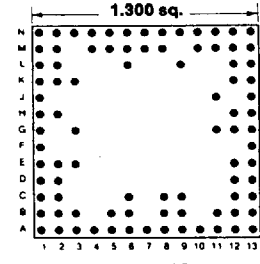
88 PINS
