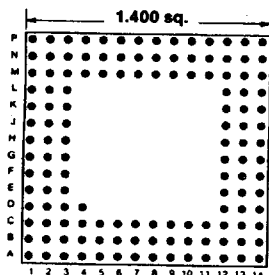
133 PINS Footprint 14014
