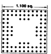
84 PINS Footprint 11010
