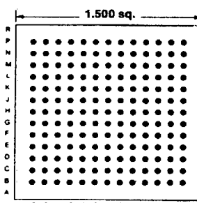
169 PINS Footprint 15036
