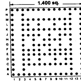
Footprint 14010
