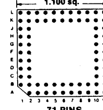
71 PINS Footprint 11027
