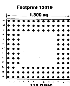
Footprint 13019
