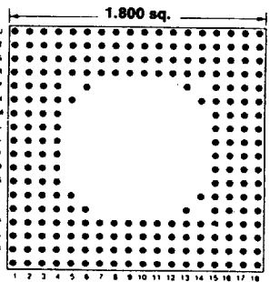
Footprint 18008
