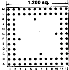
84 PINS Footprint 12011
