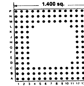
Footprint 14012
