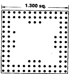
100 PINS Footprint 13059
