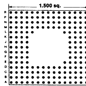
179 PINS Footprint 15012
