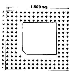
145 PINS Footprint 15023
