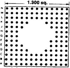
133 PINS Footprint 13052
