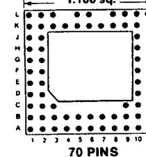
70 PINS Footprint 11028
