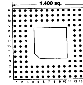
Footprint 14011
