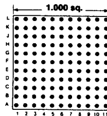
121 PINS Footprint 11001
