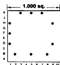
11 PINS Footprint 10011
