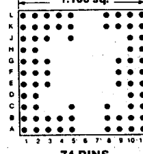
74 PINS Footprint 11018
