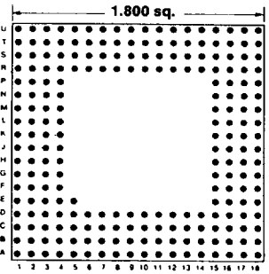
Footprint 18003
