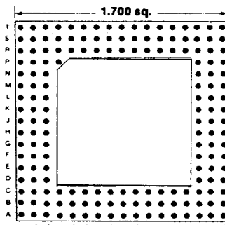
169 PINS Footprint 17010
