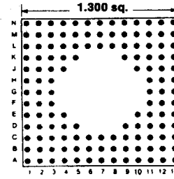
132 PINS
