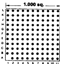
120 PINS Footprint 11002
