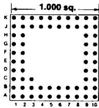
65 PINS Footprint 10008
