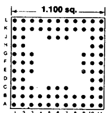
85 PINS Footprint 11008
