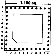
Footprint 11043
