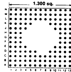
133 PINS Footprint 13055
