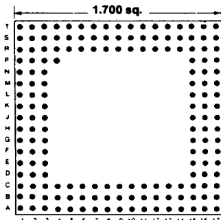
169 PINS Footprint 17002
