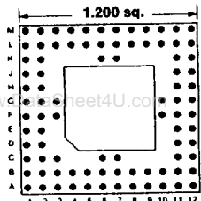
89 PINS Footprint 12006
