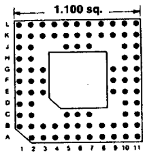
83 PINS Footprint 11013
