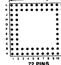
72 PINS Footprint 11024
