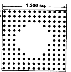
133 PINS Footprint 13054
