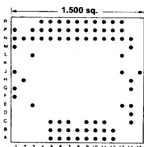
75 PINS Footprint 15032
