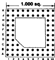
65 PINS Footprint 10007
