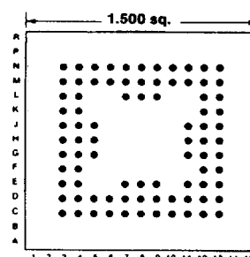
85 PINS Footprint 15034
