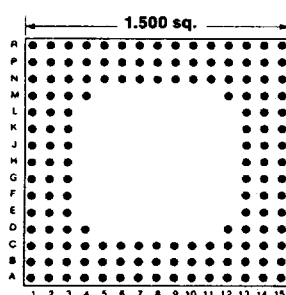
148 PINS Footprint 15022
