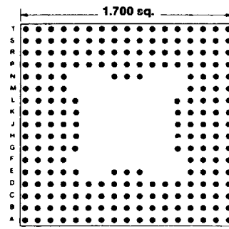
225 PINS Footprint 17008
