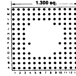
128 PINS
