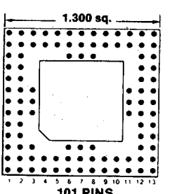
Footprint 13021
