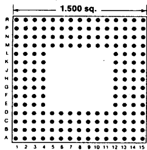
176 PINS Footprint 15014
