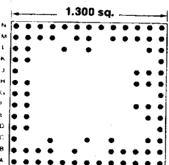
88 PINS Footprint 13057
