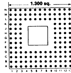
133 PINS Footprint 13004
