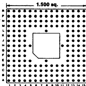
181 PINS Footprint 15005
