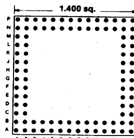
96 PINS Footprint 14024
