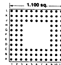
96 PINS Footprint 11006
