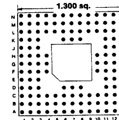
132 PINS Footprint 13006
