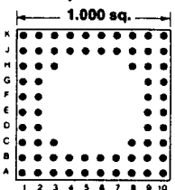
68 PINS Footprint 10006
