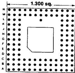
114 PINS Footprint 13051
