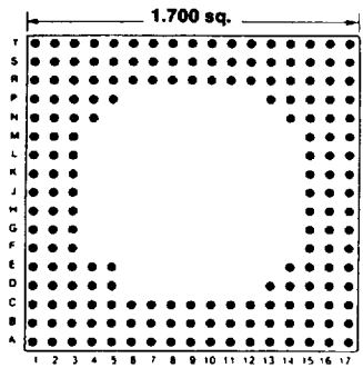
Footprint 17015
