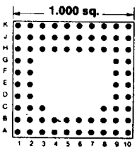
72 PINS Footprint 10004
