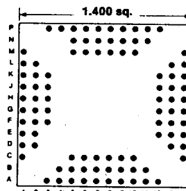
94 PINS Footprint 14023
