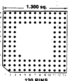
Footprint 13016
