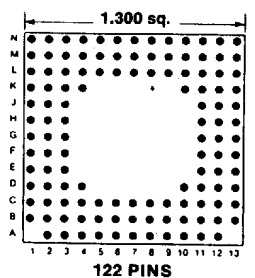
Footprint 13010
