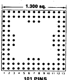
Footprint 13022
