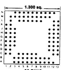
Footprint 13026
