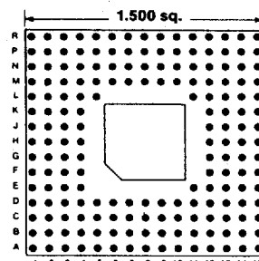
179 PINS Footprint 15011
