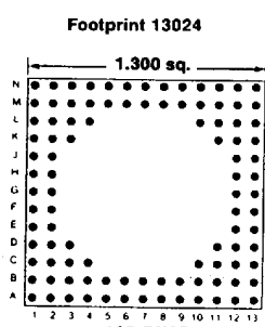
Footprint 13024
