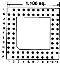
Footprint 11032
