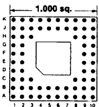
66 PINS Footprint 10005
