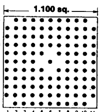
113 PINS Footprint 11004
