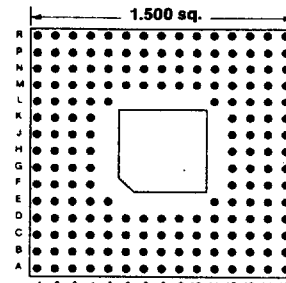
180 PINS Footprint 15009
