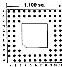
75 PINS Footprint 11015
