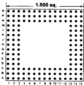
144 PINS Footprint 15026
