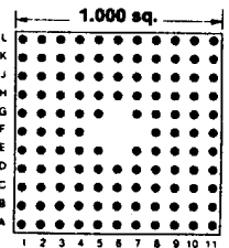
116 PINS Footprint 11003
