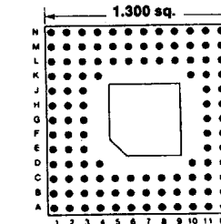
124 PINS Footprint 13008
