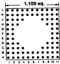
84 PINS Footprint 11012
