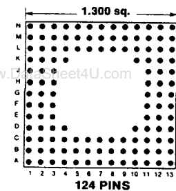
124 PINS
