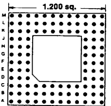
Footprint 12004
