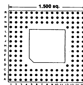
148 PINS Footprint 15021
