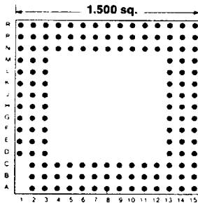
141 PINS Footprint 15029
