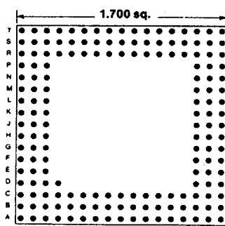
169 PINS Footprint 17012
