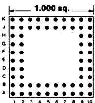
64 PINS Footprint 10010
