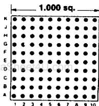
100 PINS Footprint 10001
