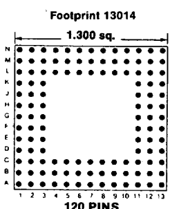
Footprint 13014
