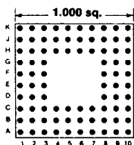
84 PINS Footprint 10003
