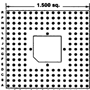
180 PINS Footprint 15007
