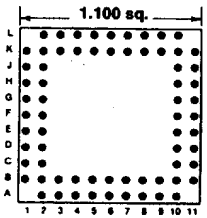
Footprint 11033
