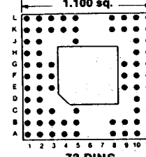
73 PINS Footprint 11019
