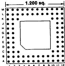
84 PINS Footprint 12012
