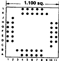
Footprint 11042
