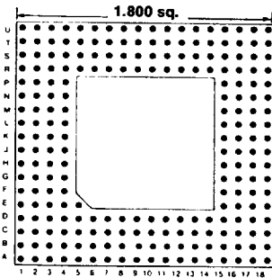
Footprint 18002
