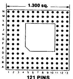
Footprint 13011
