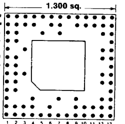
88 PINS Footprint 13049
