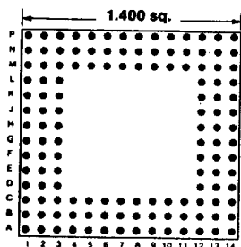
132 PINS Footprint 14016
