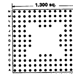
132 PINS Footprint 13007
