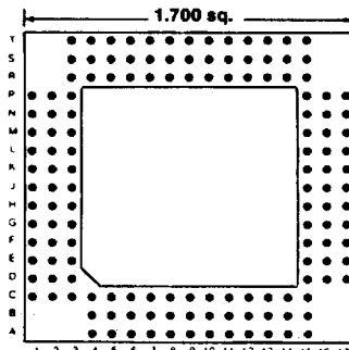
144 PINS Footprint 17005
