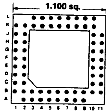
Footprint 11036
