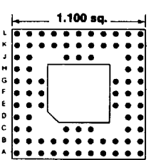
84 PINS Footprint 11009
