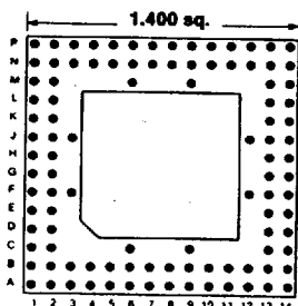
104 PINS Footprint 14017
