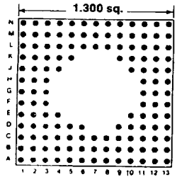
133 PINS Footprint 13046
