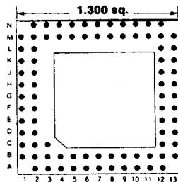
85 PINS
