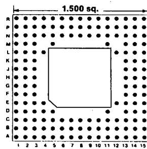
153 PINS Footprint 15016
