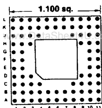
84 PINS Footprint 11011
