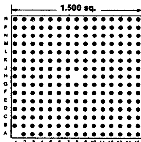
223 PINS Footprint 15003
