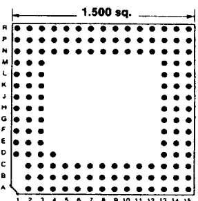
142 PINS Footprint 15027
