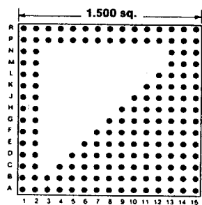
160 PINS Footprint 15015
