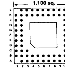
69 PINS Footprint 11030
