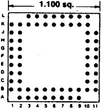
Footprint 11037
