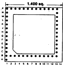
49 PINS Footprint 14019
