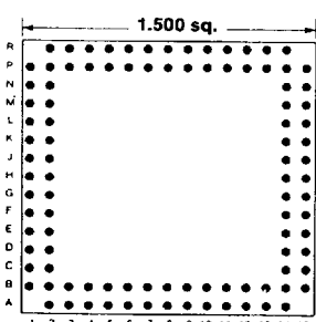
100 PINS Footprint 15031
