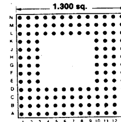
133 PINS Footprint 13005
