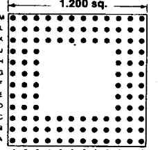
Footprint 12005
