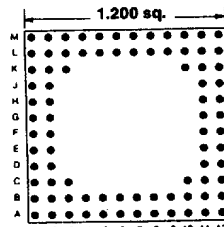
84 PINS Footprint 12013
