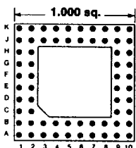
64 PINS Footprint 10009
