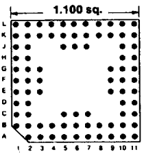
83 PINS Footprint 11014
