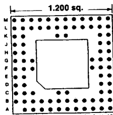
88 PINS Footprint 12008
