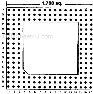
Footprint 17013
