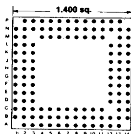
125 PINS Footprint 14021
