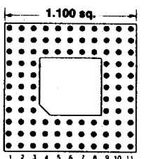
96 PINS Footprint 11005
