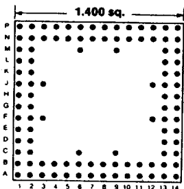
104 PINS Footprint 14018
