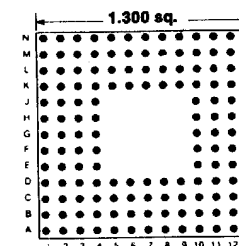
144 PINS Footprint 13003
