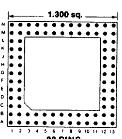
Footprint 13027
