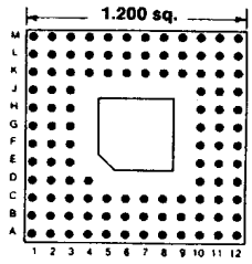
Footprint 12002
