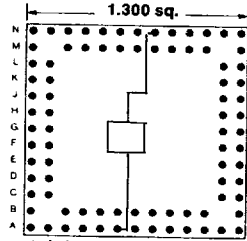
84 PINS Footprint 13056
