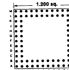
80 PINS Footprint 12015
