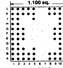
73 PINS Footprint 11020
