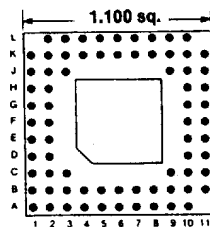
73 PINS Footprint 11021
