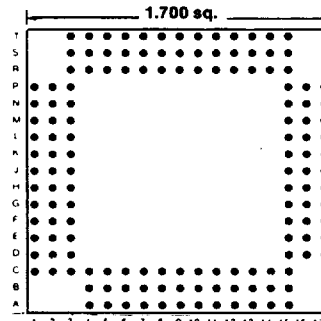
144 PINS Footprint 17006
