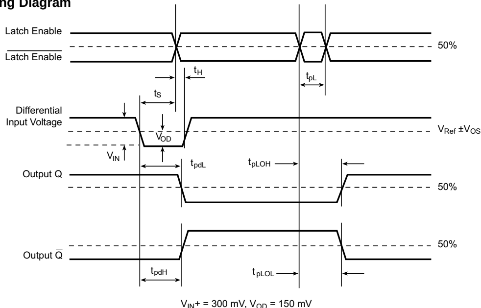
Figure 4 – Timing Diagram
