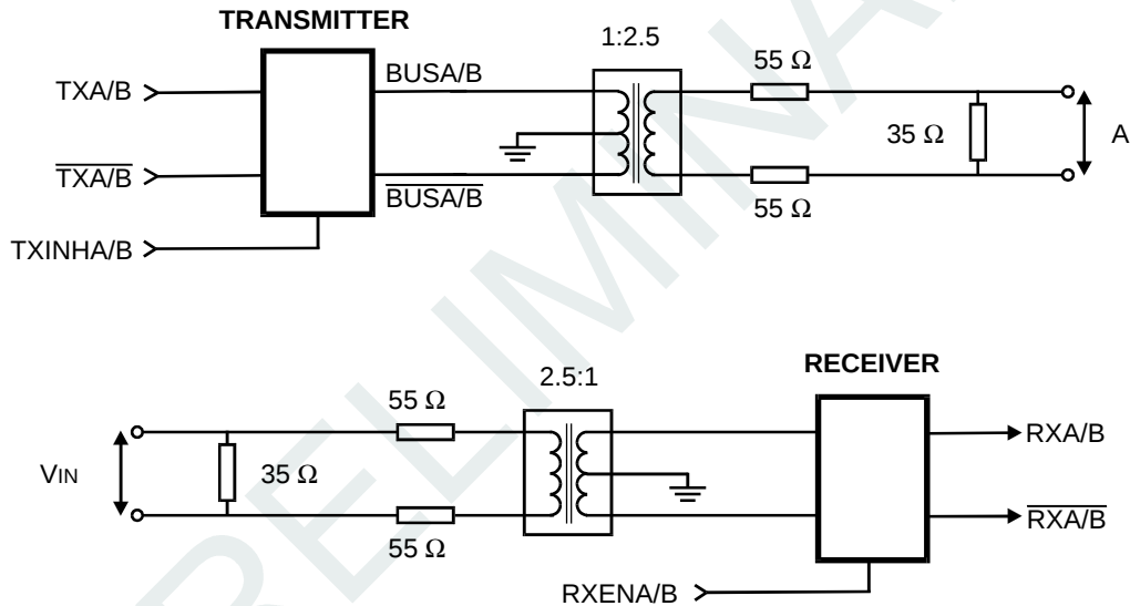
Figure 2. Test circuit
