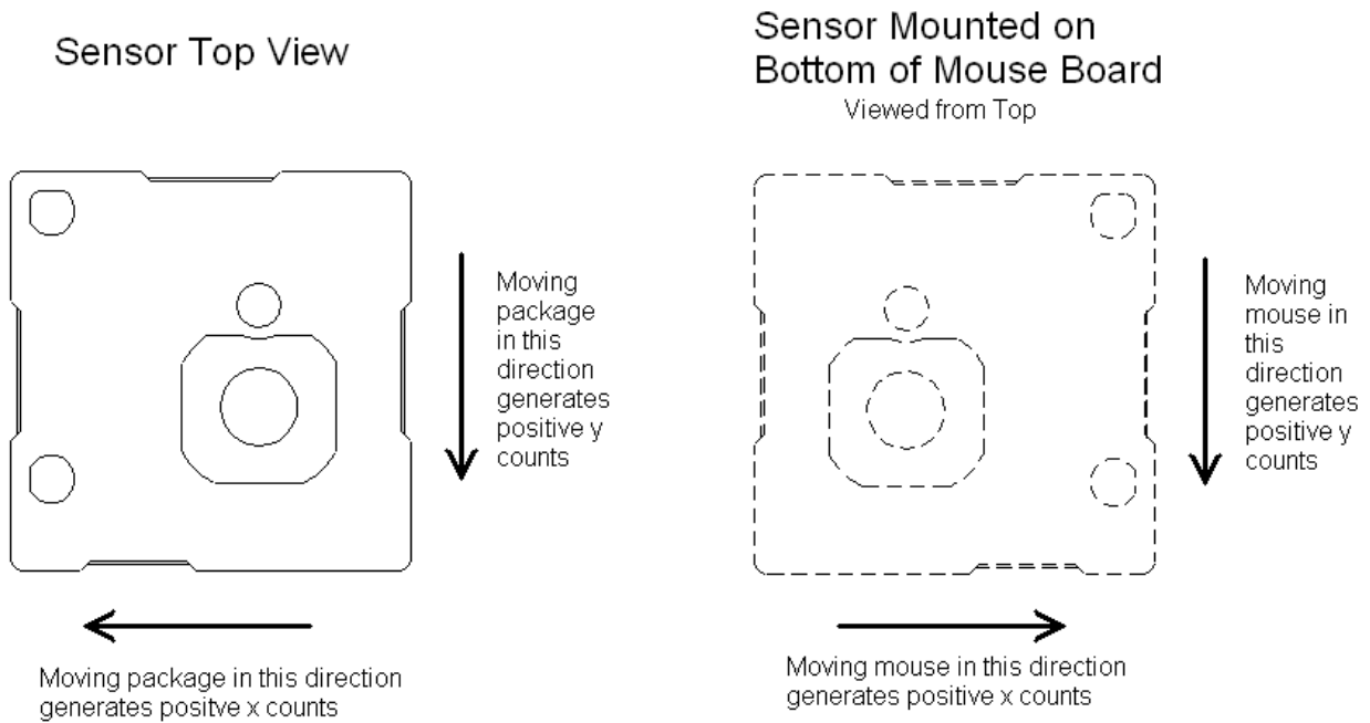
Figure 14. Sensor Orientation
