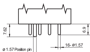
Terminal style 2 (Solder pin)
