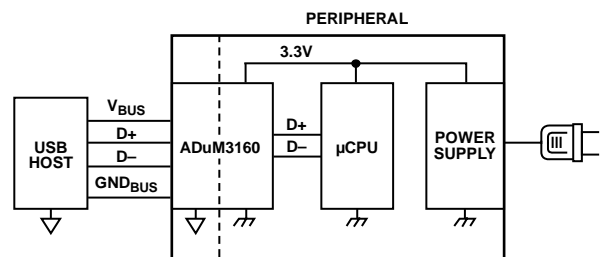
Figure 4. Typical ADuM3160 Application
