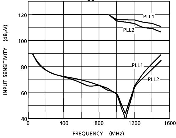
INPUT SENSITIVITY CHARACTERISTICS V CC = 3.8V
