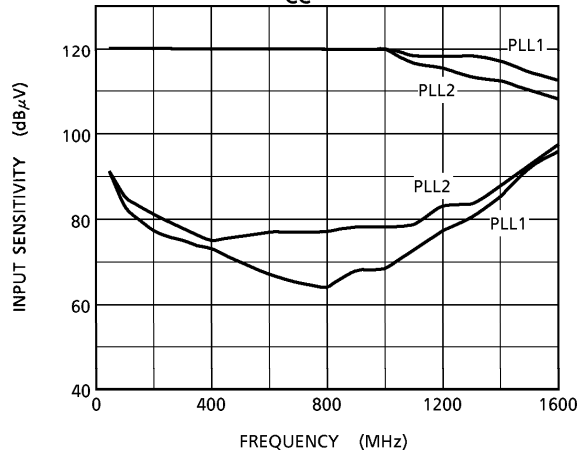
INPUT SENSITIVITY CHARACTERISTICS V CC = 3.8V
