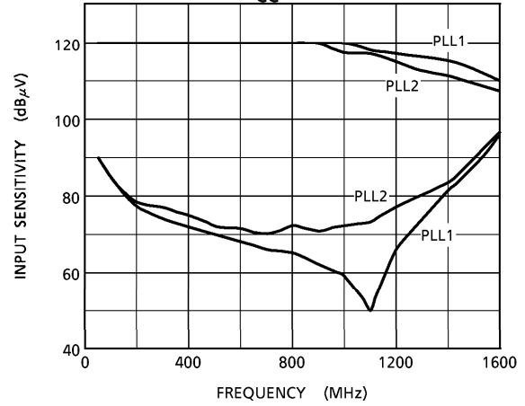
INPUT SENSITIVITY CHARACTERISTICS V CC = 3.0V
