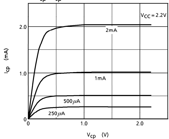
V cp -I cp CHARACTERISTICS PLL2 Nch
