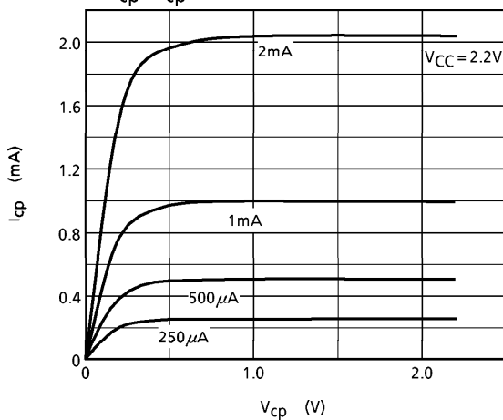
V cp -I cp CHARACTERISTICS PLL1 Nch
