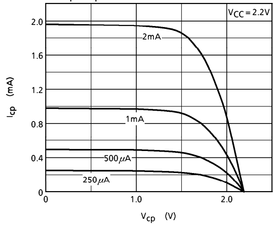
V cp -I cp CHARACTERISTICS PLL2 Pch
