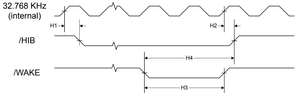
Figure 23-4. Hibernation Module Timing
