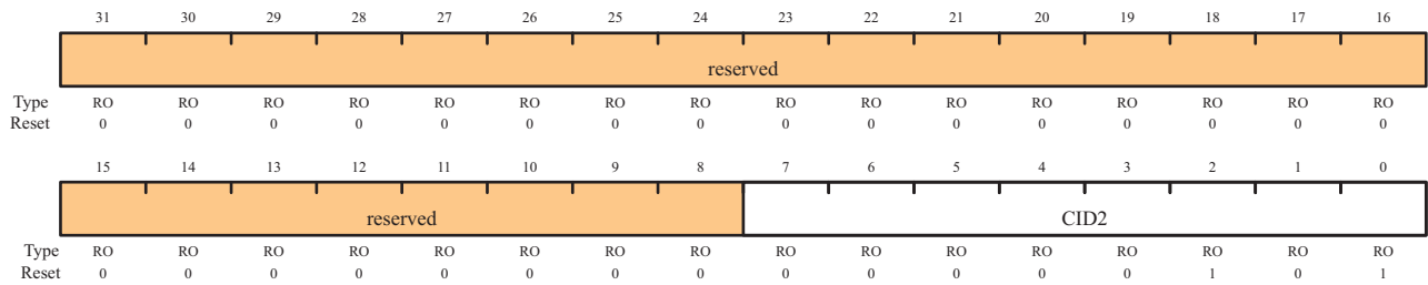
Watchdog Primecell Identification 2 (WDTPCellID2)
