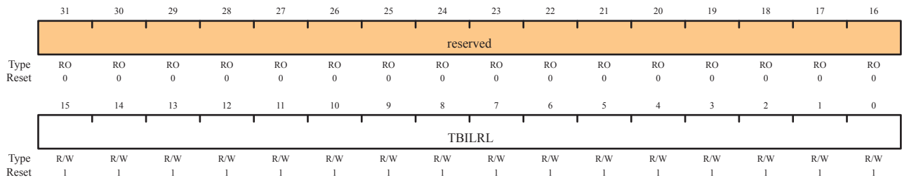
GPTM TimerB Interval Load (GPTMTBILR)
