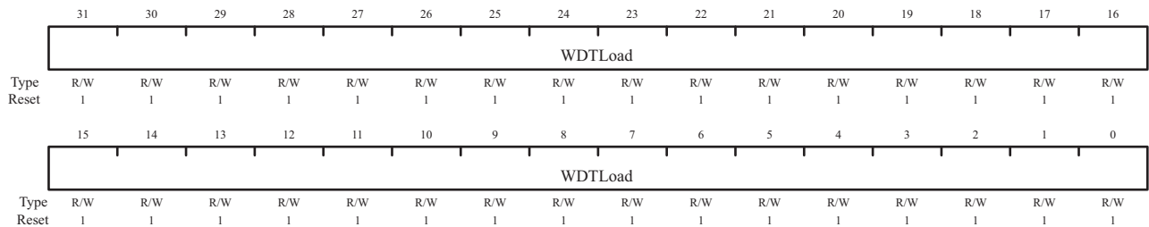
Watchdog Load (WDTLOAD) Offset 0x000
