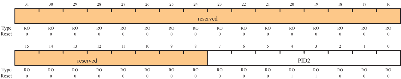
GPIO Peripheral Identification 2 (GPIOPeriphID2)
