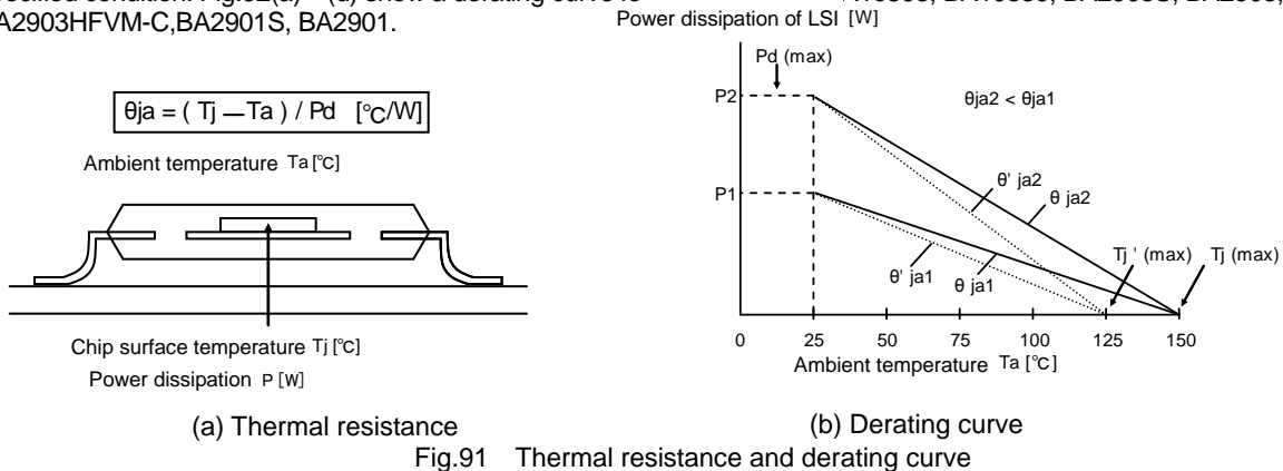
Fig.91 Thermal resistance and derating curve
