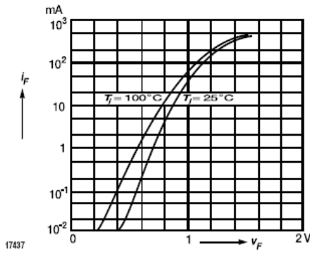
Figure 1. Forward characteristics
