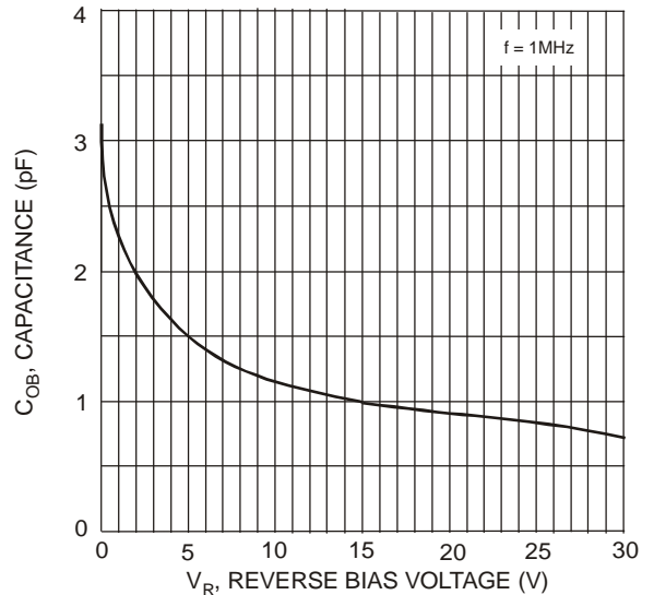
Fig. 4 Output Capacitance
