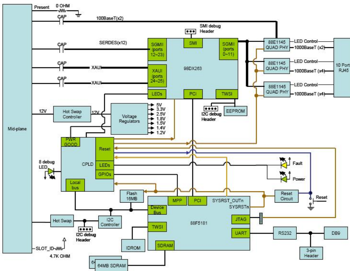
Figure 20. Ethernet Switch Module Block Diagram
