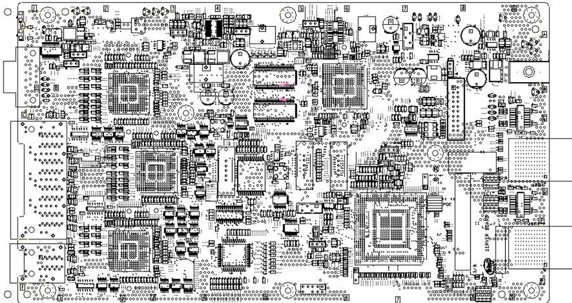
Figure 19. Ethernet Switch Module Mechanical Outline (Top View)
