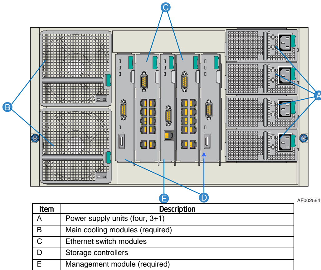
Figure 4. Rear View of Server Platform
