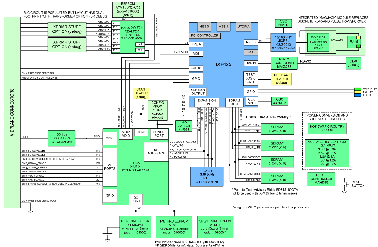
Figure 17. Chassis Management Module Block Diagram
