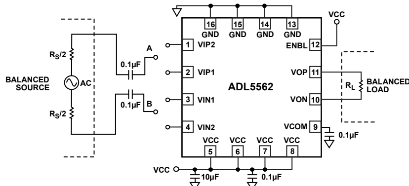
Figure 31. Basic Connections
