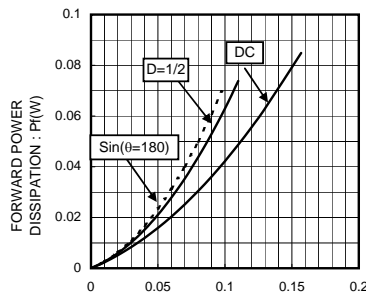
AVERAGE RECTIFIED FORWARD CURRENT : I_o (A) I_o - P_R CHARACTERISTICS
