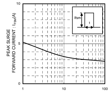
TIME : t (ms) I_{FSM} - t CHARACTERISTICS
