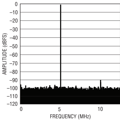
LTC2170-12: 8k Point FFT, f_{IN} = 5\text{MHz} -1\text{dBFS} , 25Mps
