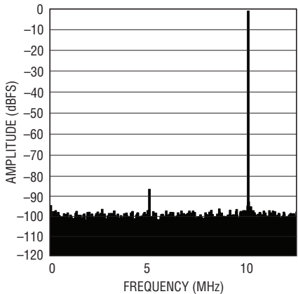
LTC2170-12: 8k Point FFT, f_{IN} = 140\text{MHz} -1\text{dBFS} , 25Mps
