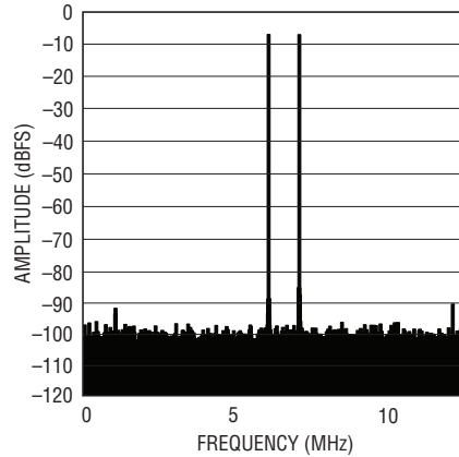
LTC2170-12: 8k Point 2-Tone FFT, f_{IN} = 68\text{MHz} , 69\text{MHz} , -1\text{dBFS} , 25Mps
