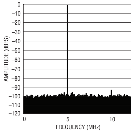
LTC2170-12: 8k Point FFT, f_{IN} = 30\text{MHz} -1\text{dBFS} , 25Mps
