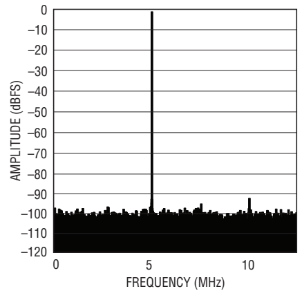
LTC2170-12: 8k Point FFT, f_{IN} = 70\text{MHz} -1\text{dBFS} , 25Mps
