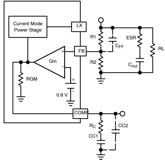
Figure 4. NCP1599 Compensation Components
