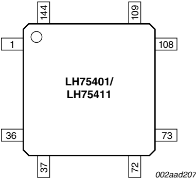
Figure 3. LH75401/LH75411 pin configuration
