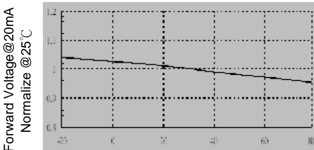
Fig.3 Forward Voltage vs. Temperature
