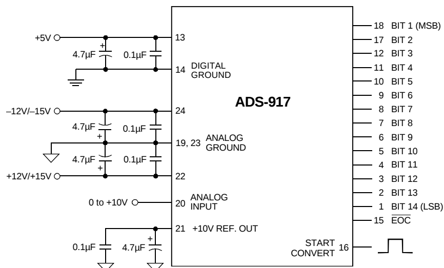
Figure 3. Typical ADS-917 Connection Diagram
