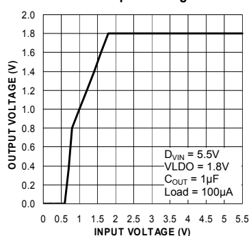
LDO Output Voltage vs. Input Voltage
