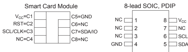
Figure 1. Package Options
