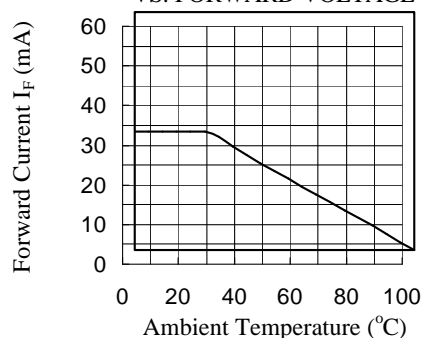
FIG.4 FORWARD CURRENT VS. AMBIENT TEMPERATURE
