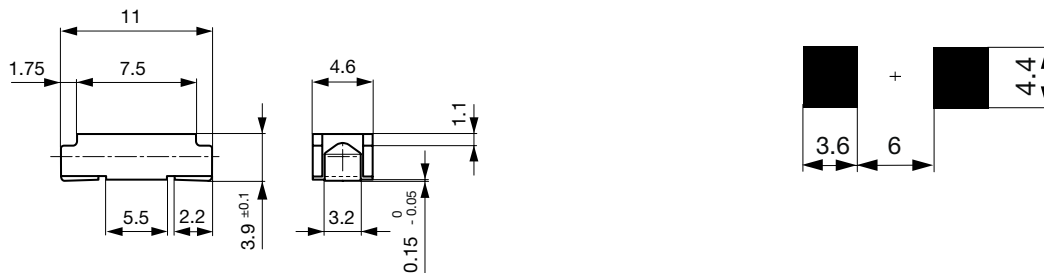
Soldering pads
