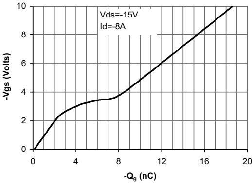
Figure 7: Gate-Charge Characteristics
