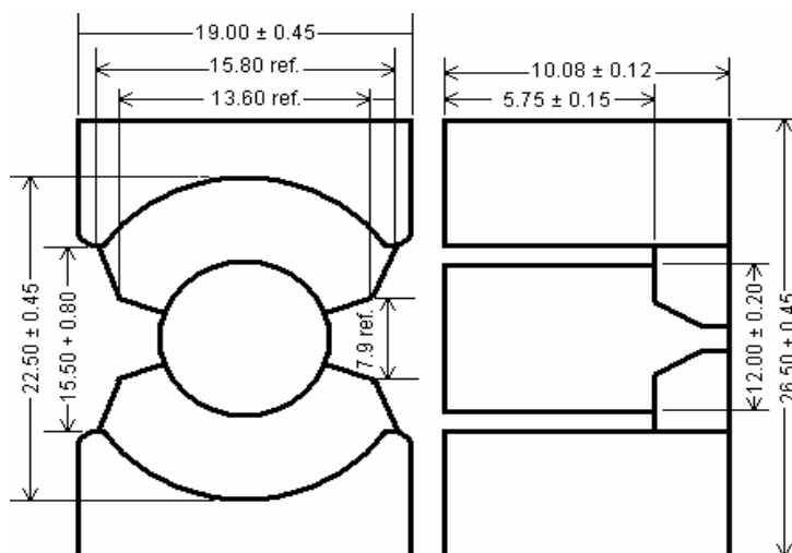
Dimensions (mm)
