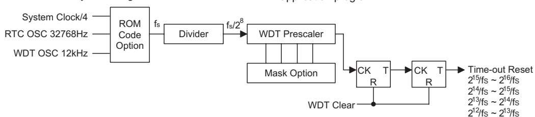
Watchdog Timer
