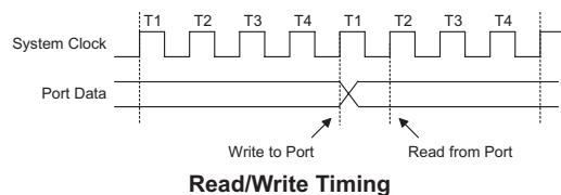
Read/Write Timing
