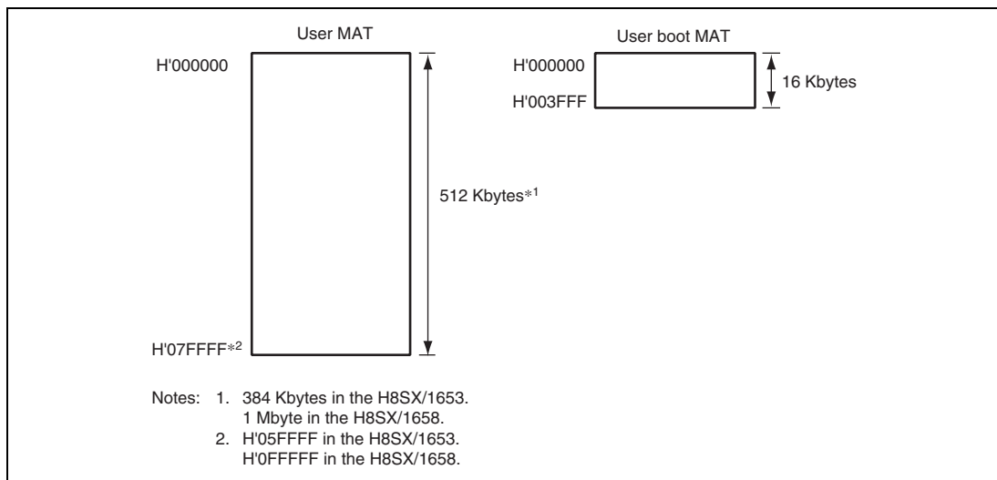
Figure 24.3 Memory MAT Configuration (H8SX/1654)
