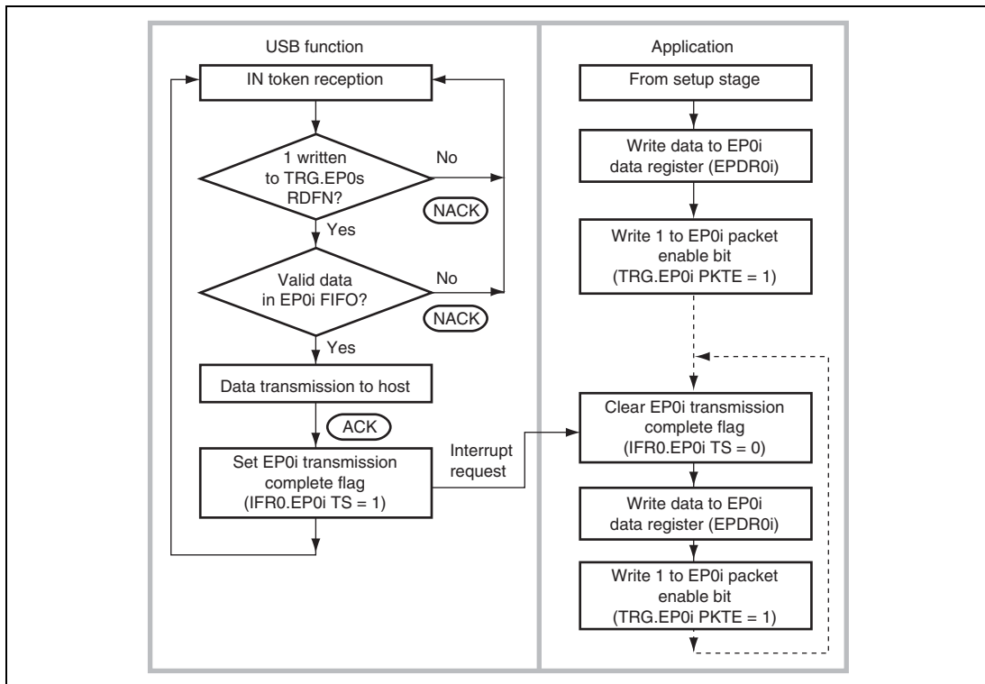
Figure 19.13 Data Stage (Control-In) Operation
