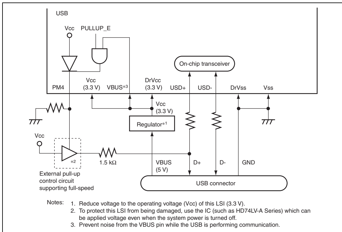
Figure 19.24 Example of Circuitry in Bus Power Mode
