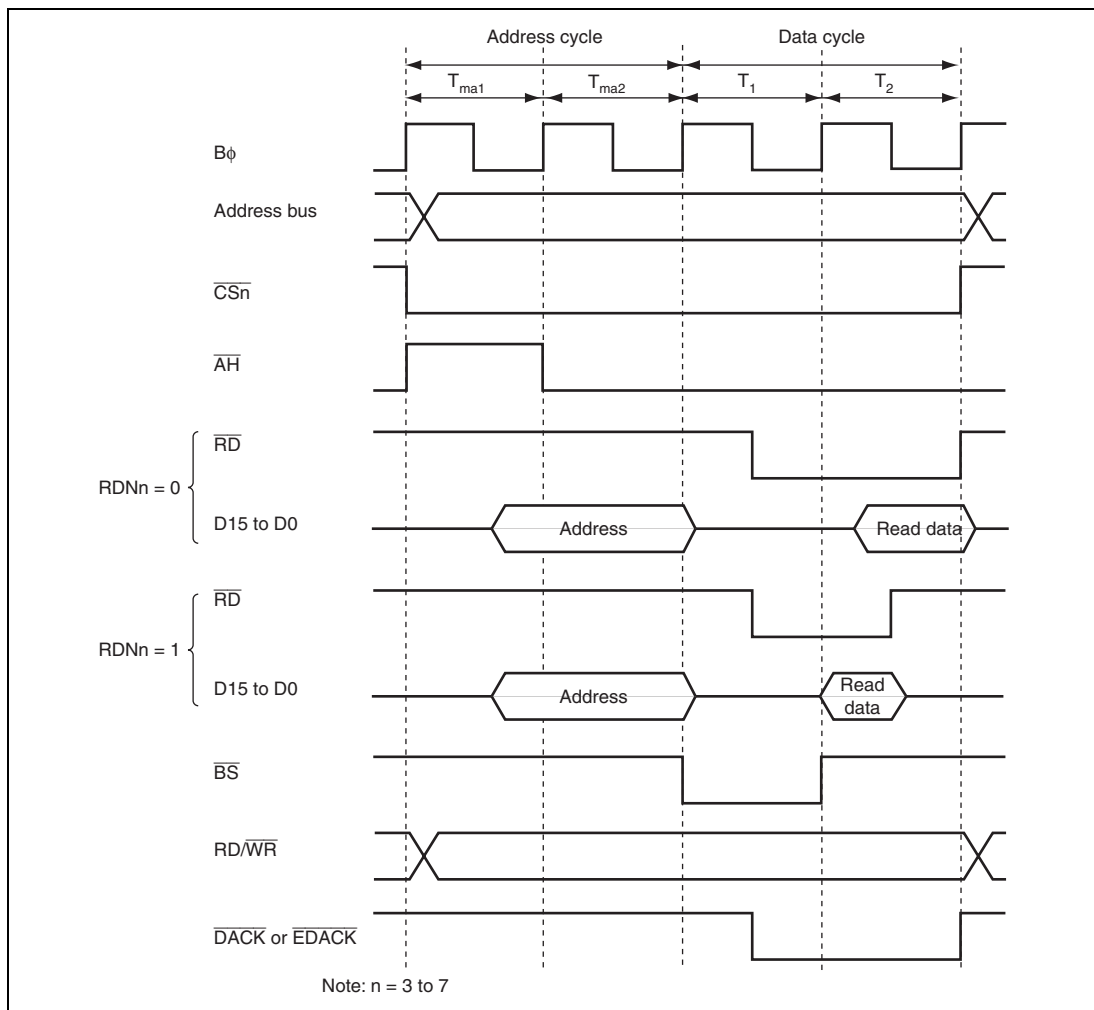
Figure 9.33 Read Strobe Timing
