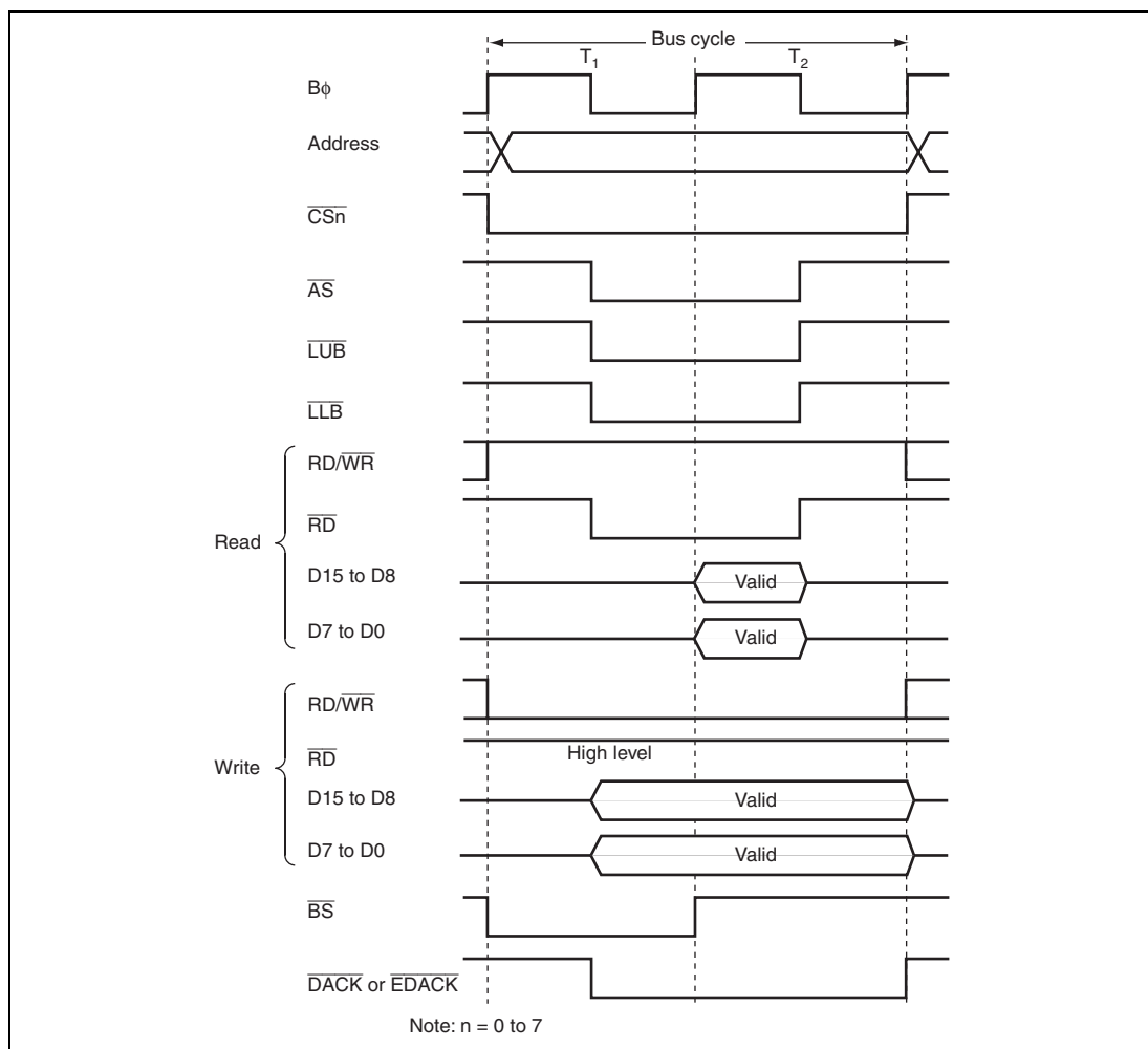
Figure 9.24 16-Bit 2-State Access Space Bus Timing
