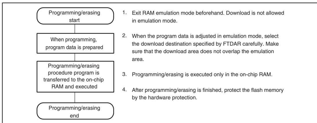
Figure 24.11 Programming/Erasing Flow
