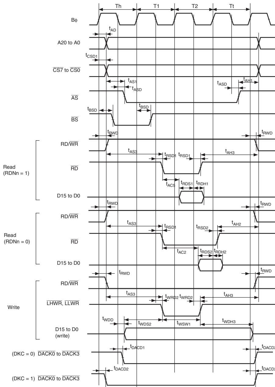
Figure 29.11 Basic Bus Timing: Two-State Access ( \overline{\text{CS}} Assertion Period Extended)
