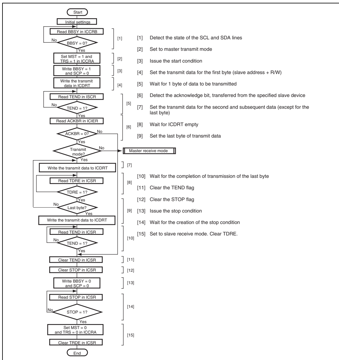
Figure 20.14 Sample Flowchart of Master Transmit Mode
