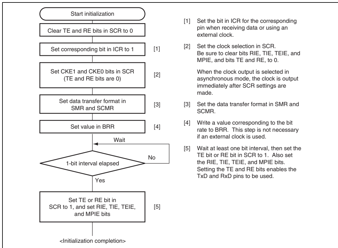
Figure 18.8 Sample SCI Initialization Flowchart
