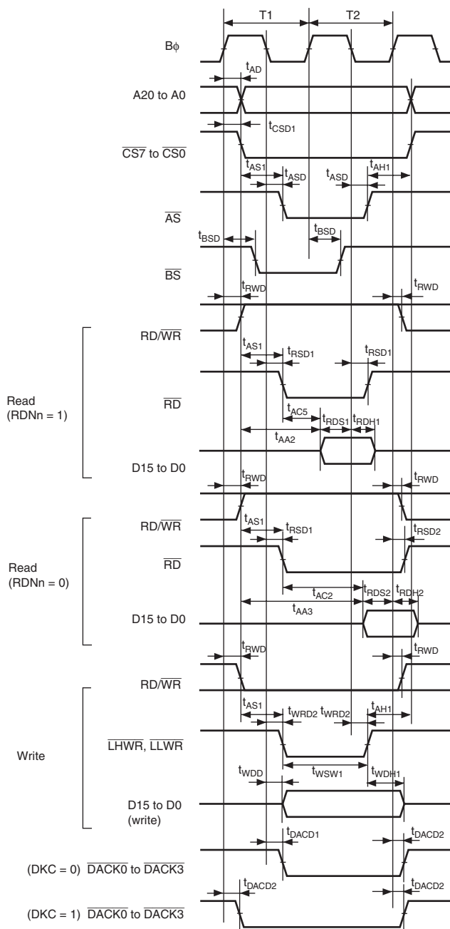
Figure 29.8 Basic Bus Timing: Two-State Access
