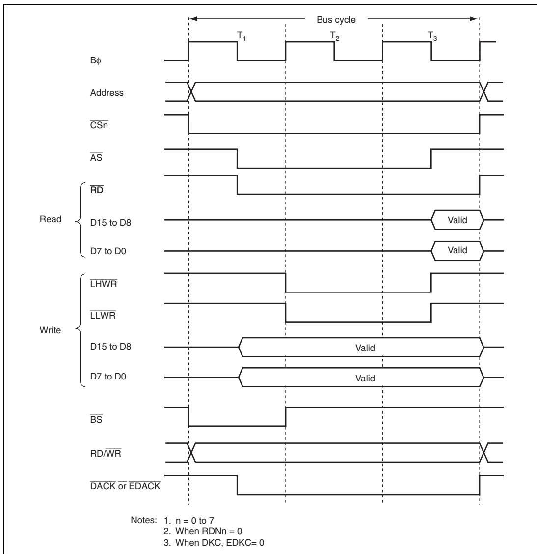
Figure 9.19 16-Bit 3-State Access Space Bus Timing (Word Access for Even Address)
