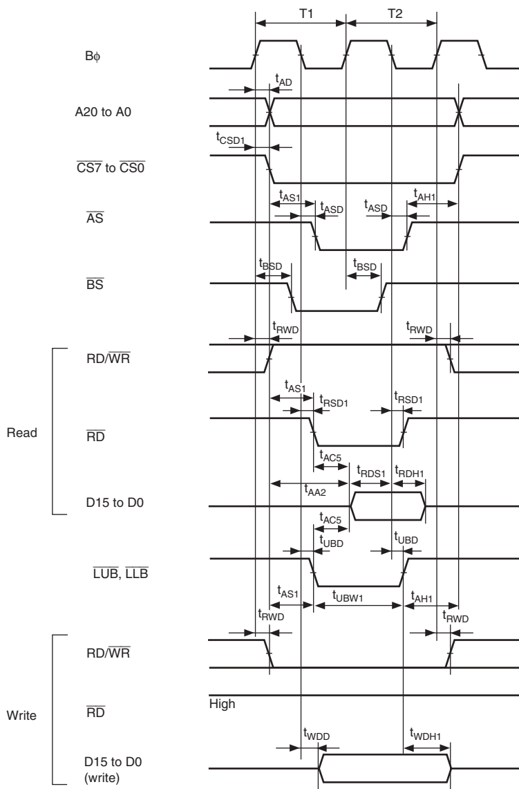
Figure 29.13 Byte Control SRAM: Two-State Read/Write Access
