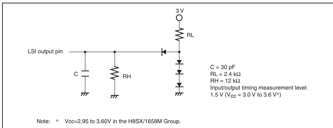
Figure 29.1 Output Load Circuit
