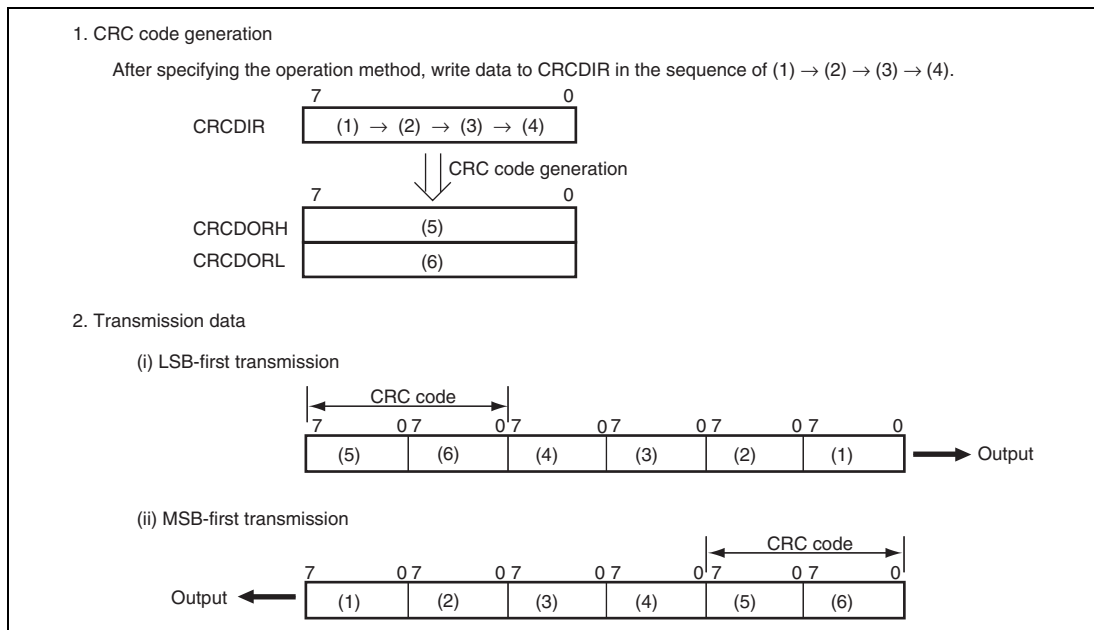
Figure 18.48 LSB-First and MSB-First Transmit Data
