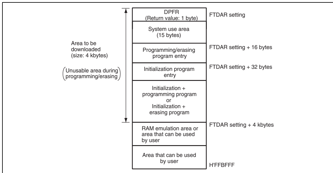
Figure 24.12 RAM Map when Programming/Erasure is Executed
