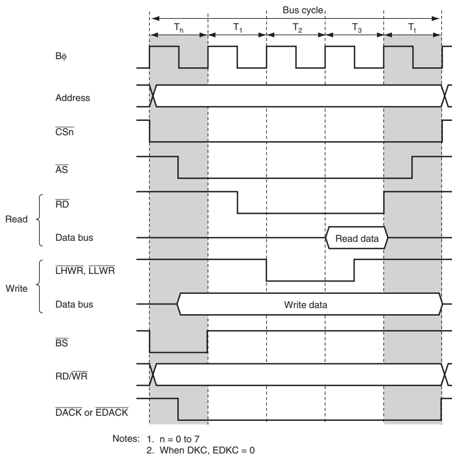
Figure 9.22 Example of Timing when Chip Select Assertion Period is Extended
