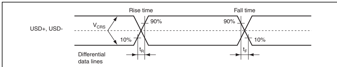
Figure 29.41 Data Signal Timing
