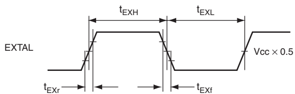
Figure 29.5 External Input Clock Timing
