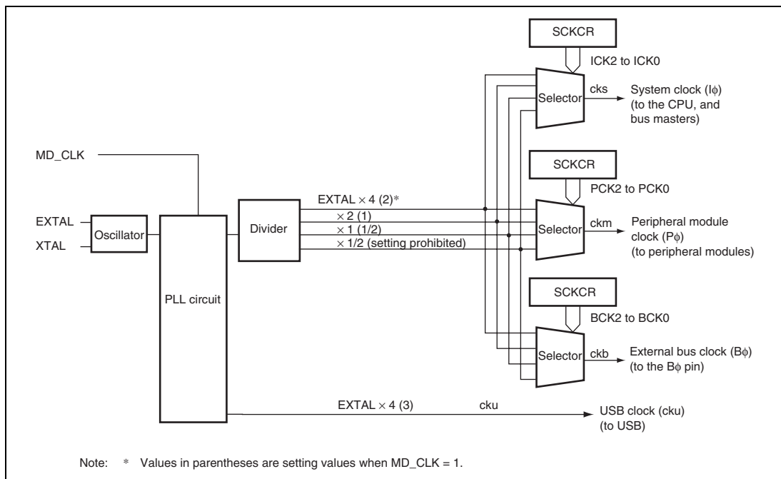
Figure 26.1 Block Diagram of Clock Pulse Generator
