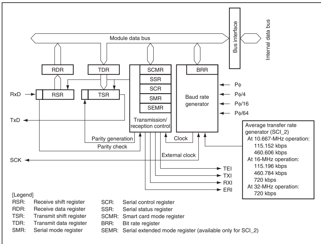
Figure 18.1 Block Diagram of SCI_0, 1, 2, and 4
