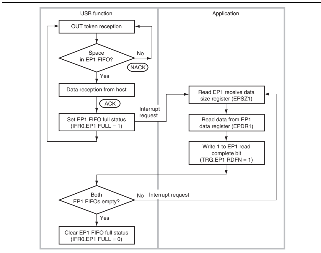
Figure 19.17 EP1 Bulk-Out Transfer Operation
