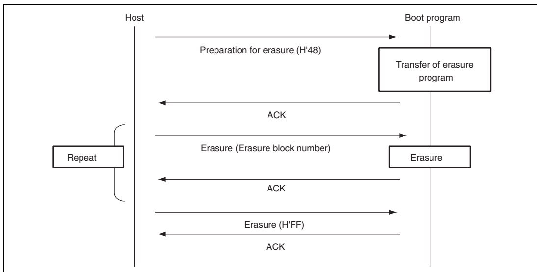
Figure 28.26 Erasure Sequence
