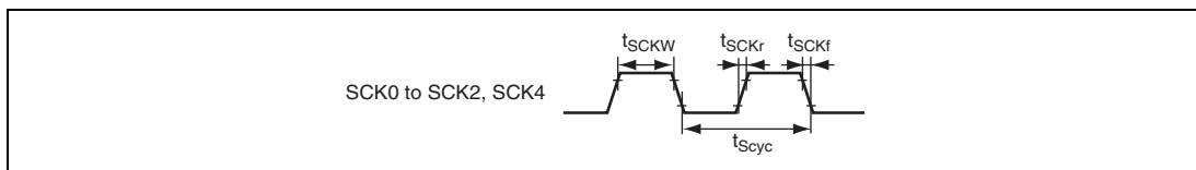
Figure 29.34 SCK Clock Input Timing
