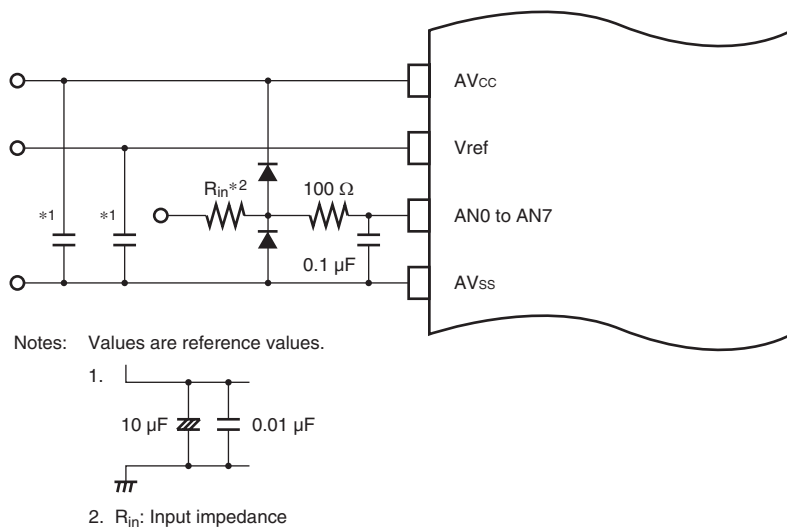
Figure 21.13 Example of Analog Input Protection Circuit
