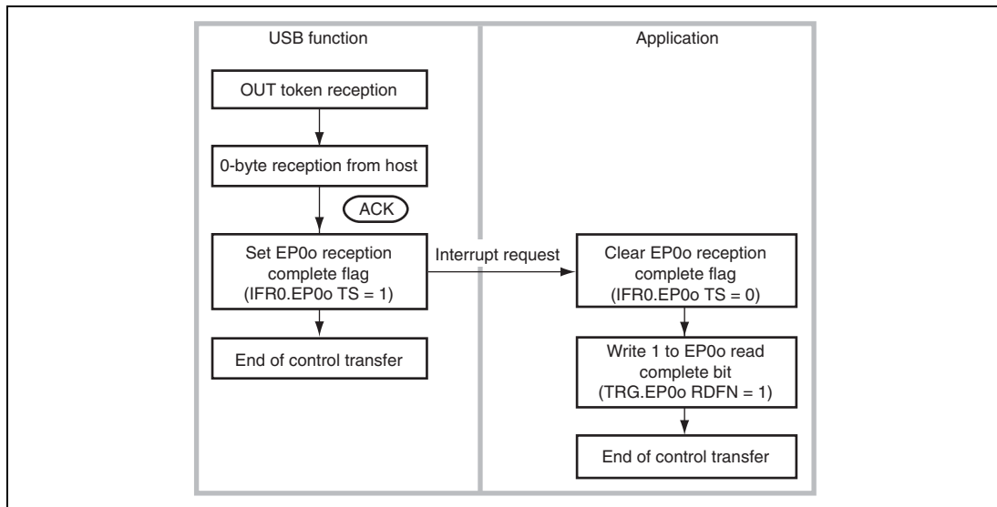
Figure 19.15 Status Stage (Control-In) Operation
