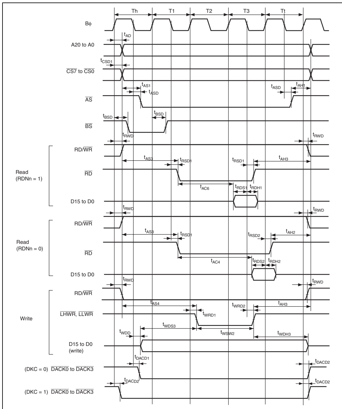
Figure 29.12 Basic Bus Timing: Three-State Access ( \overline{\text{CS}} Assertion Period Extended)
