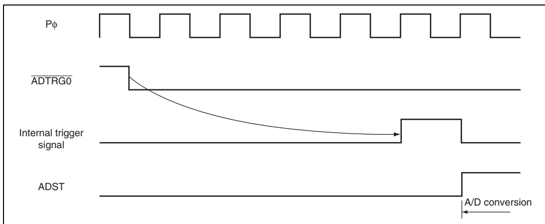
Figure 21.8 External Trigger Input Timing when Multiple Units Start Simultaneously ( TRGS1 , TRGS0 , and EXTRGS = B'111 )
