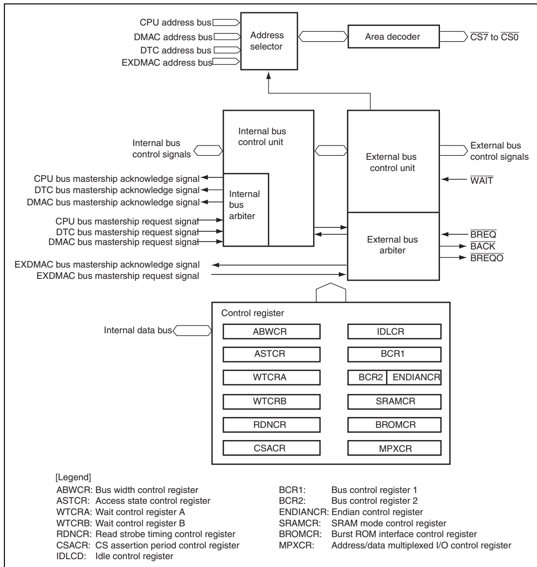
Figure 9.1 Block Diagram of Bus Controller
