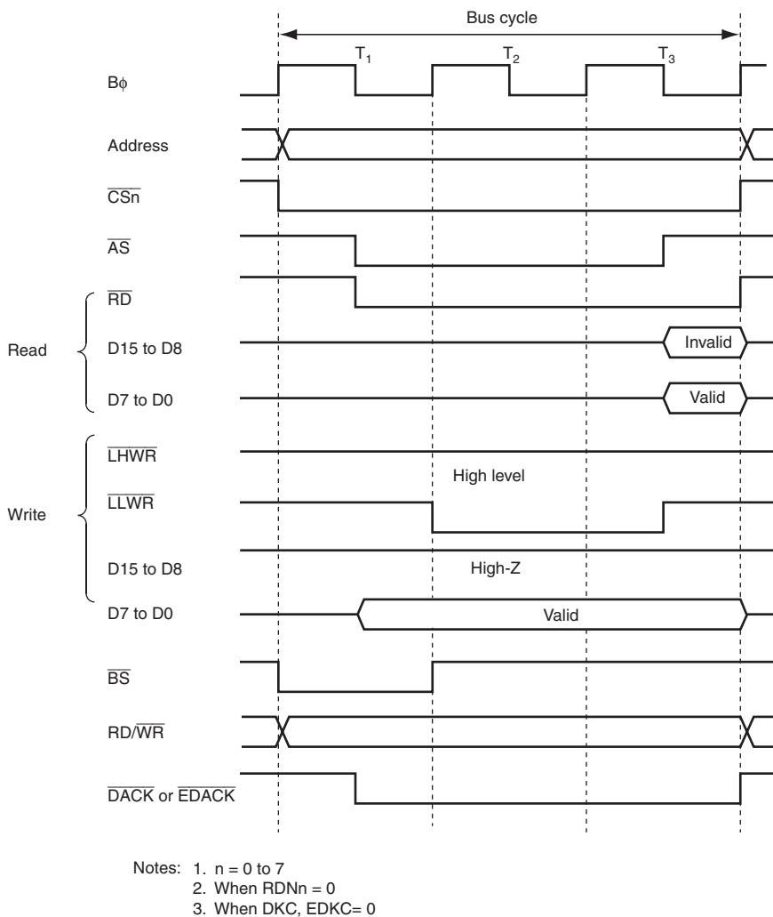
Figure 9.18 16-Bit 3-State Access Space Bus Timing (Word Access for Odd Address)
