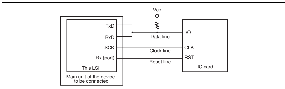
Figure 18.24 Pin Connection for Smart Card Interface
