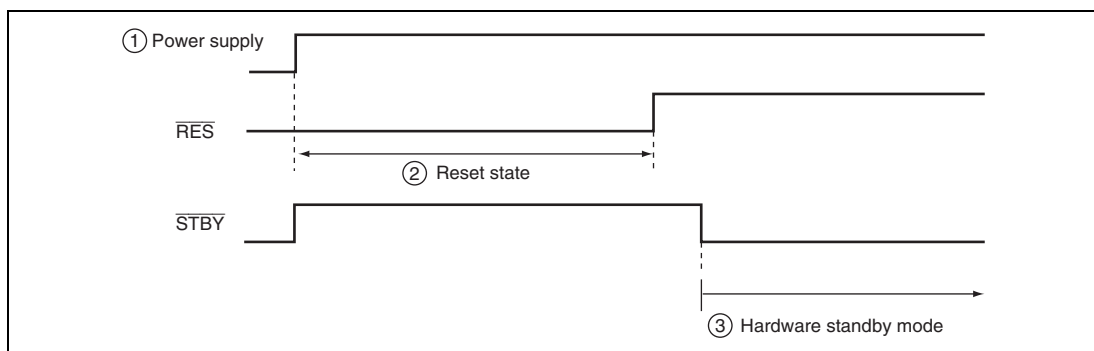
Figure 27.9 Timing Sequence at Power-On
