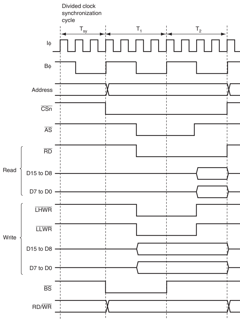
Figure 9.5 System Clock: External Bus Clock = 4:1, External 2-State Access
