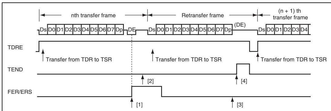
Figure 18.29 Data Re-Transfer Operation in SCI Transmission Mode
