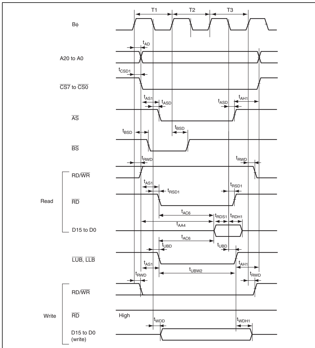
Figure 29.14 Byte Control SRAM: Three-State Read/Write Access
