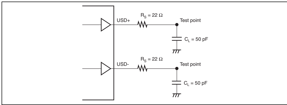
Figure 29.42 Load Condition
