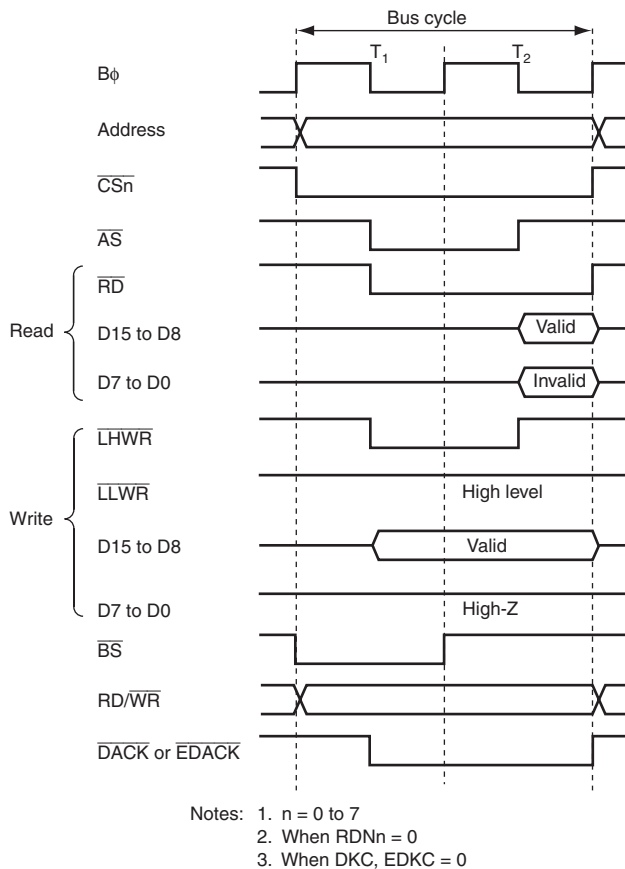
Figure 9.14 16-Bit 2-State Access Space Bus Timing (Byte Access for Even Address)
