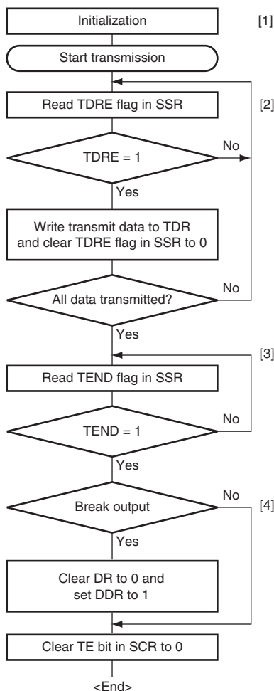
Figure 18.10 Example of Serial Transmission Flowchart
