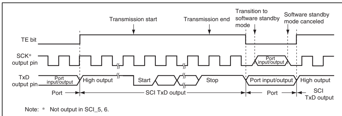
Figure 18.40 Port Pin States during Software Standby Mode Transition (Internal Clock, Asynchronous Transmission)
