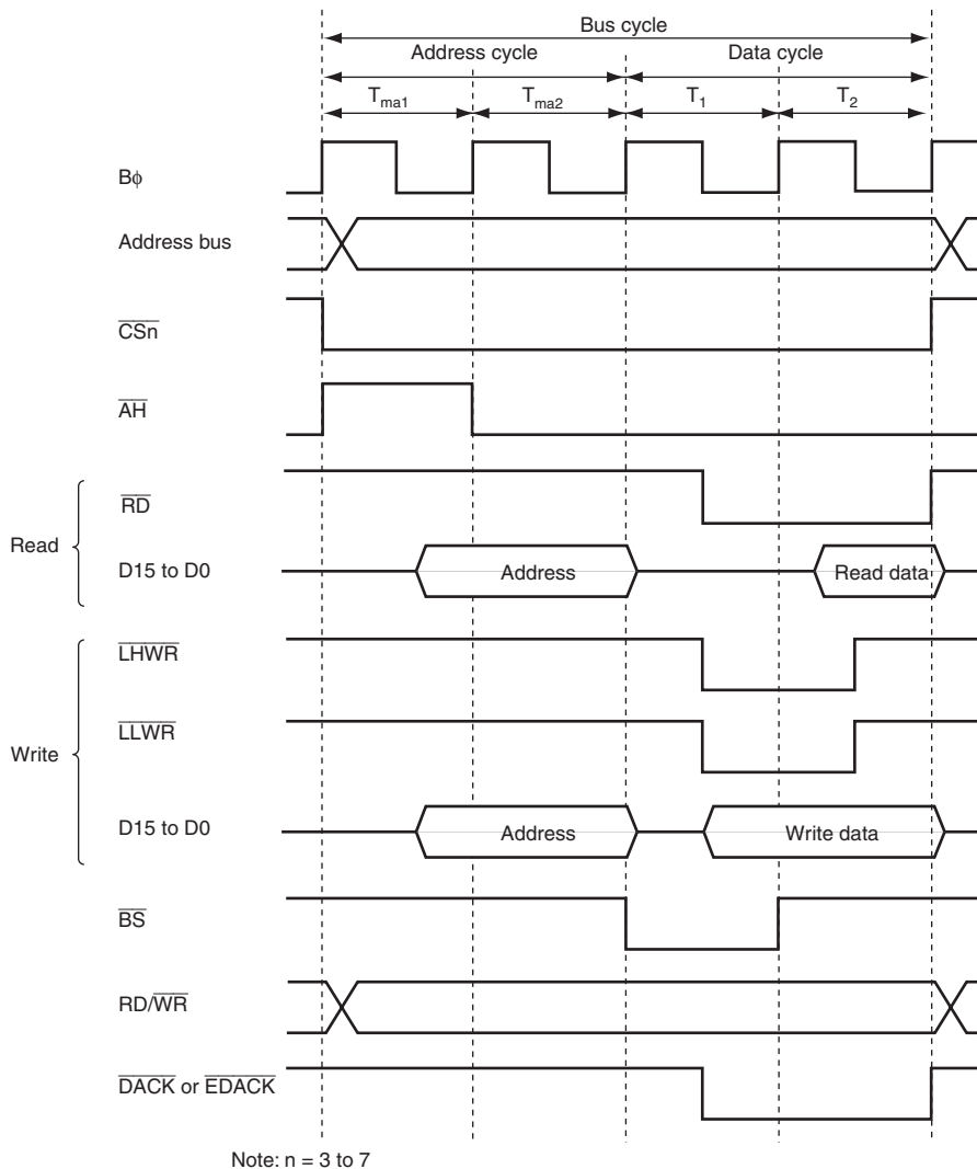
Figure 9.31 16-Bit Access Space Access Timing (ABWHn = 0, ABWLn = 1)
