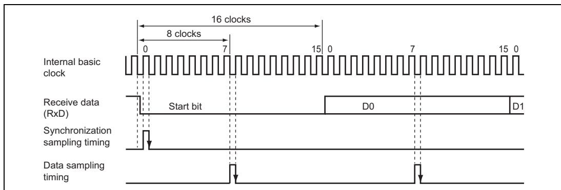
Figure 18.6 Receive Data Sampling Timing in Asynchronous Mode
