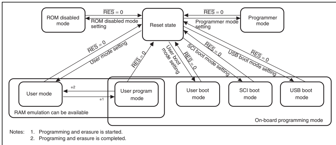
Figure 24.2 Mode Transition of Flash Memory
