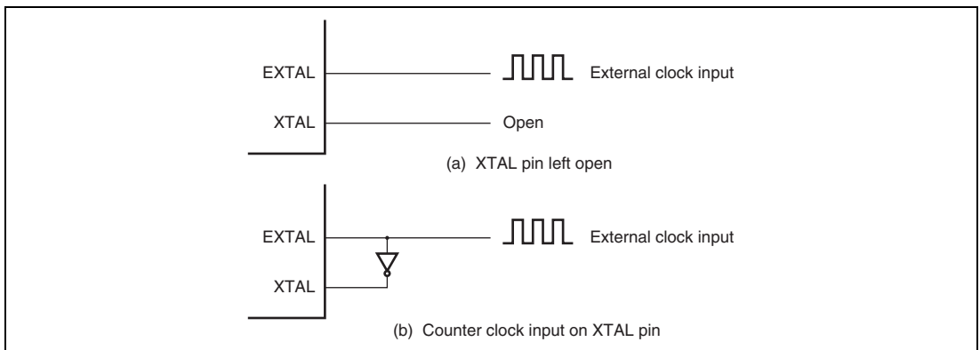
Figure 26.4 External Clock Input (Examples)
