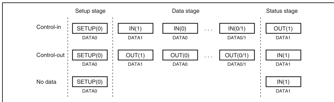
Figure 19.11 Transfer Stages in Control Transfer
