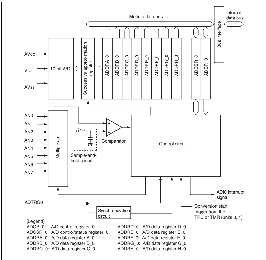
Figure 21.1 Block Diagram of A/D Converter Unit 0 (AD_0)
