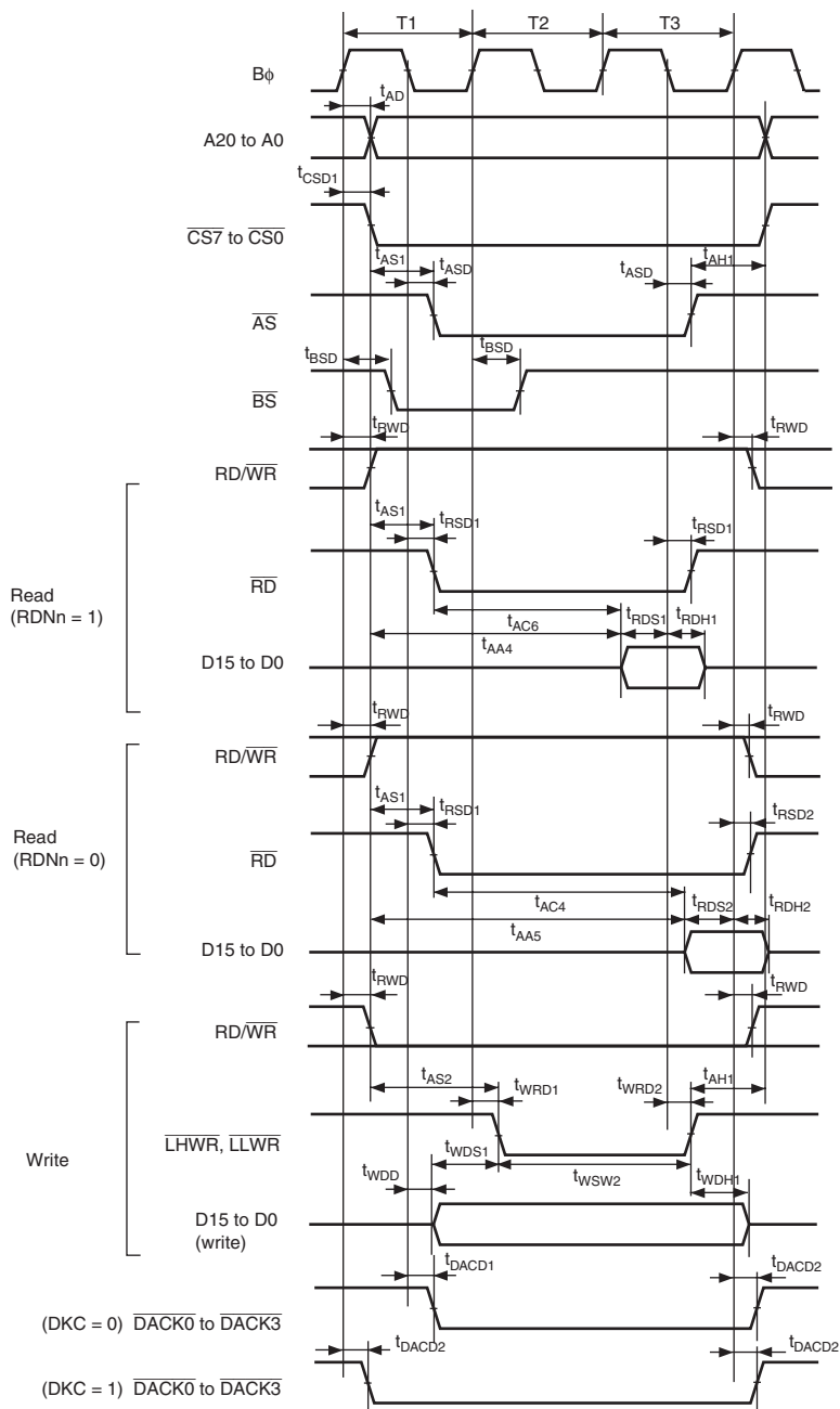
Figure 29.9 Basic Bus Timing: Three-State Access
