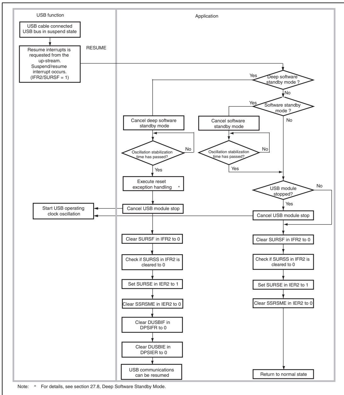
Figure 19.5 Resume Operation from Up-Stream
