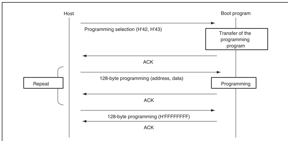
Figure 24.27 Programming Sequence
