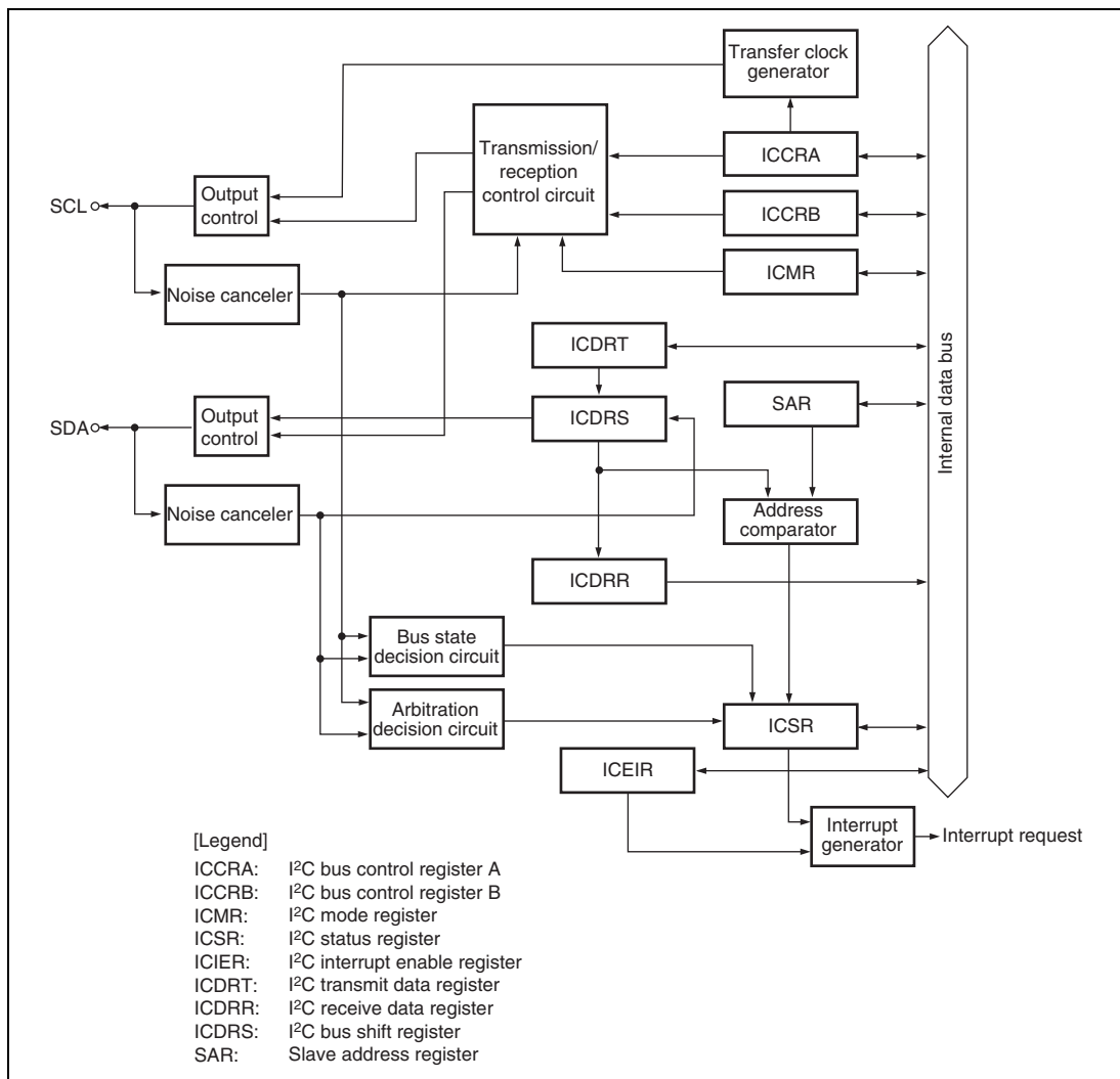
Figure 20.1 Block Diagram of I 2 C Bus Interface 2
