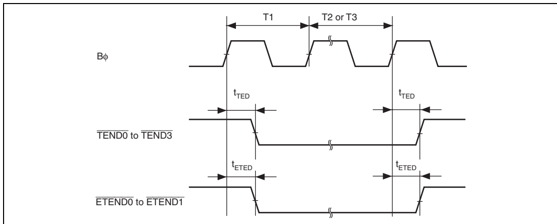
Figure 29.22 DMAC/EXDMAC ( \overline{TEND} and \overline{ETEND} ) Output Timing
