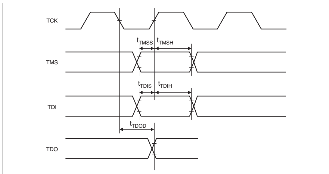
Figure 29.40 Boundary Scan Input/Output Timing
