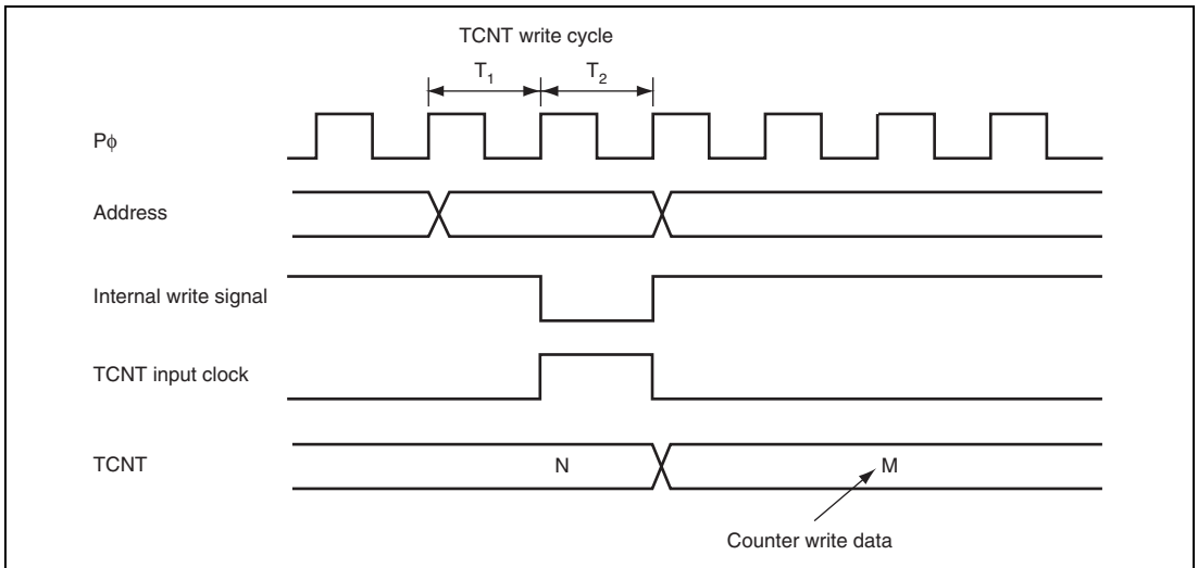
Figure 17.5 Conflict between TCNT Write and Increment
