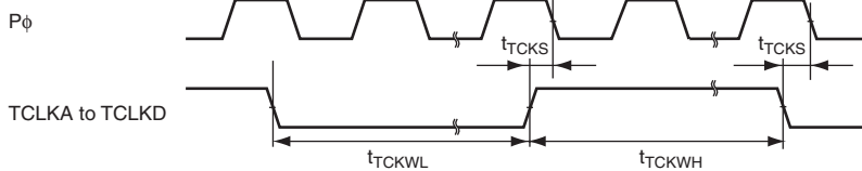
Figure 29.28 TPU Clock Input Timing
