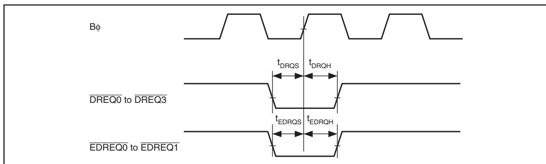
Figure 29.21 DMAC/EXDMAC ( \overline{DREQ} and \overline{EDREQ} ) Input Timing
