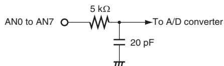
Figure 21.14 Analog Input Pin Equivalent Circuit
