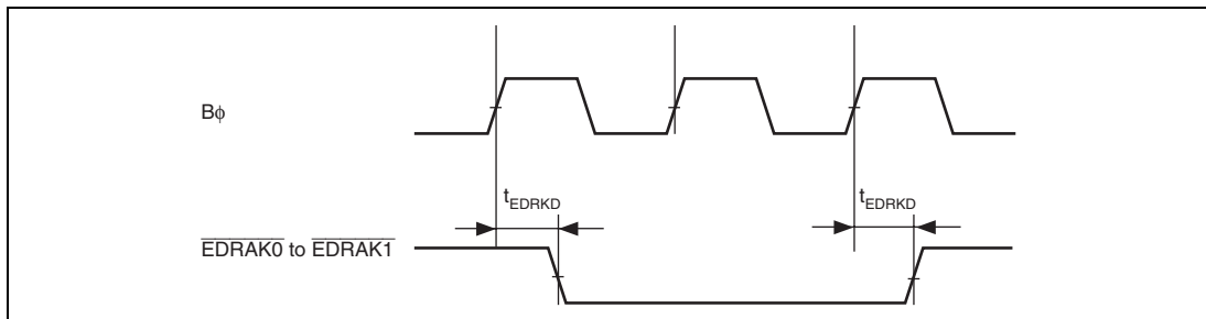
Figure 29.25 EXDMAC ( \overline{EDRAK} ) Output Timing
