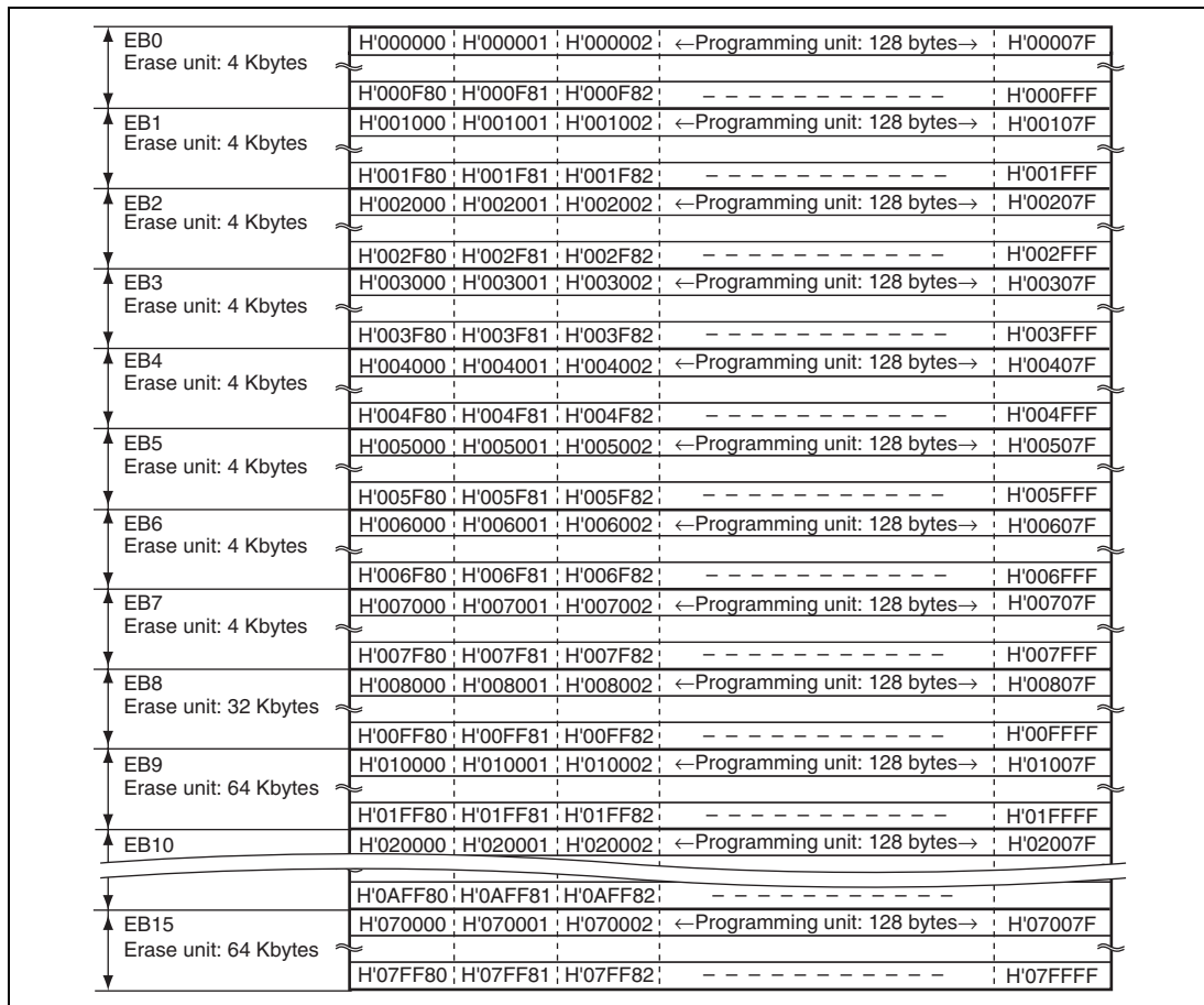
Figure 24.4 (2) User MAT Block Structure of H8SX/1654
