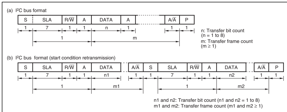
Figure 20.3 I 2 C Bus Formats
