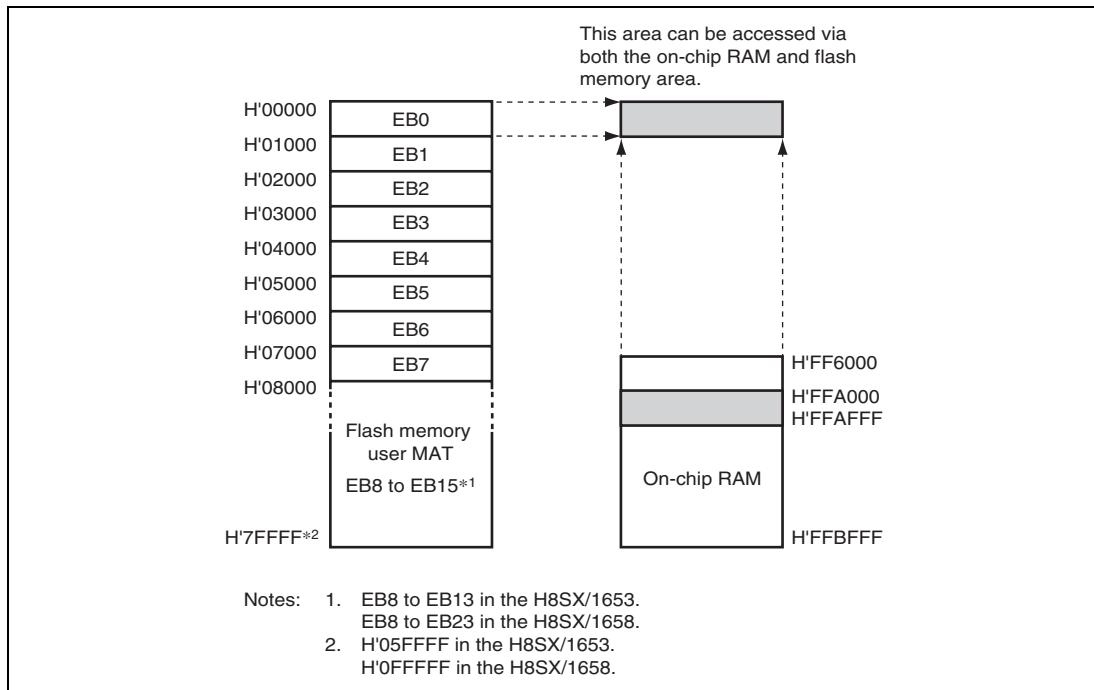
Figure 24.20 Address Map of Overlaid RAM Area (H8SX/1654)
