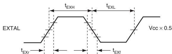
Figure 26.5 External Clock Input Timing
