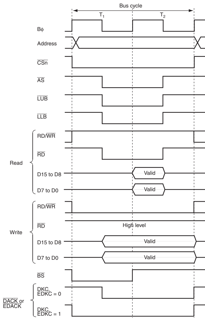
Figure 9.27 \overline{\text{DACK}} and \overline{\text{EDACK}} Signal Output Timings
