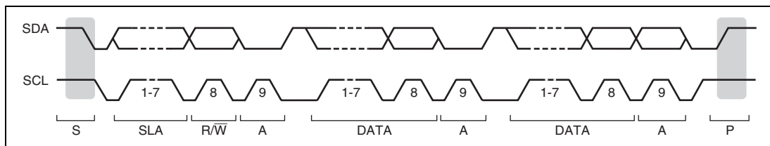
Figure 20.4 I 2 C Bus Timing
