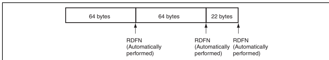
Figure 19.22 RDFN Bit Operation for EP1
