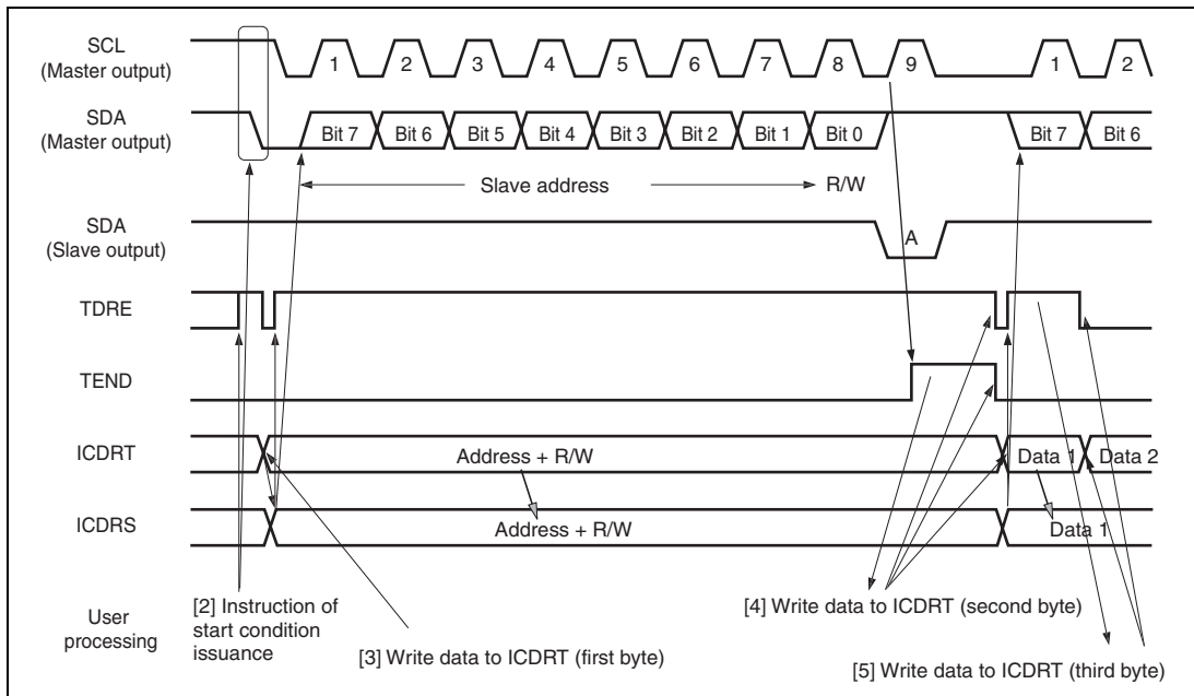
Figure 20.5 Master Transmit Mode Operation Timing 1
