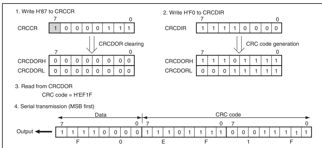
Figure 18.45 MSB-First Data Transmission
