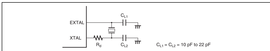
Figure 26.2 Connection of Crystal Resonator (Example)
