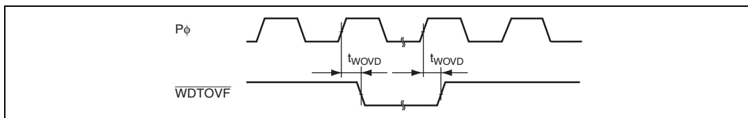
Figure 29.33 WDT Output Timing
