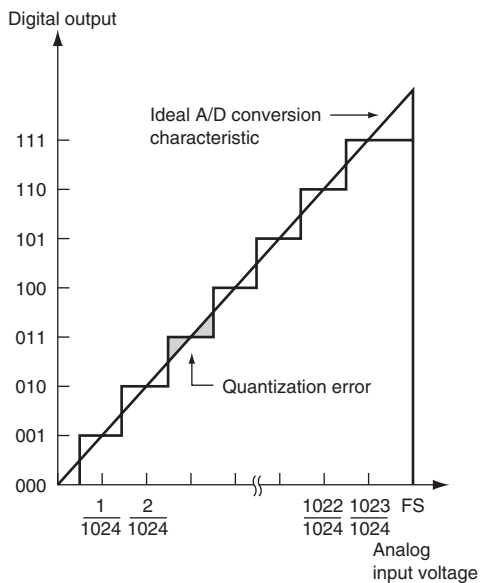
Figure 21.9 A/D Conversion Accuracy Definitions
