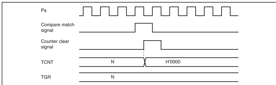
Figure 14.35 Counter Clear Timing (Compare Match)
