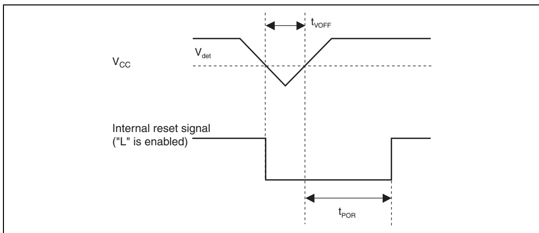
Figure 29.44 Voltage Detection Circuit Timing
