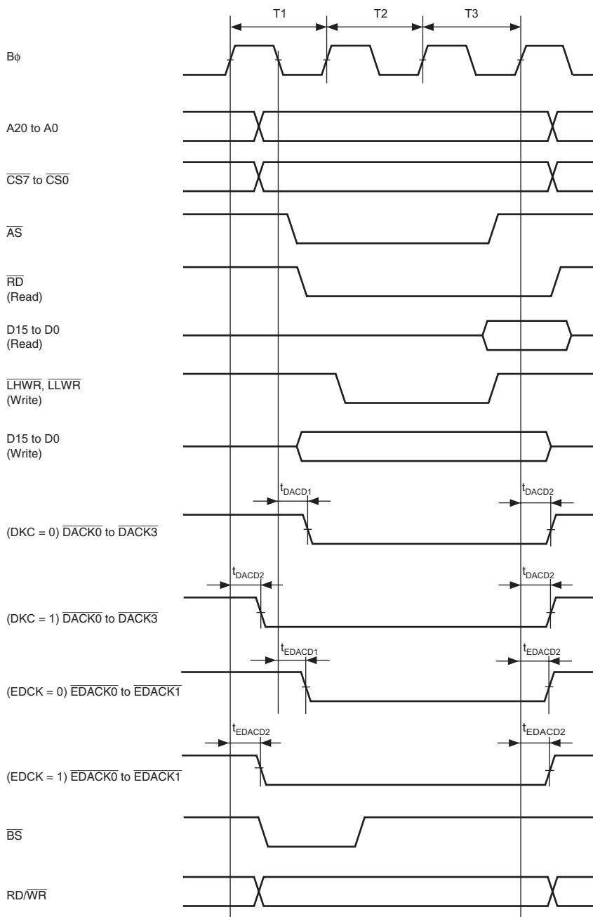
Figure 29.24 DMAC/EXDMAC Single-Address Transfer Timing: Three-State Access
