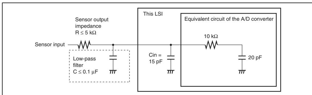
Figure 21.12 Example of Analog Input Circuit
