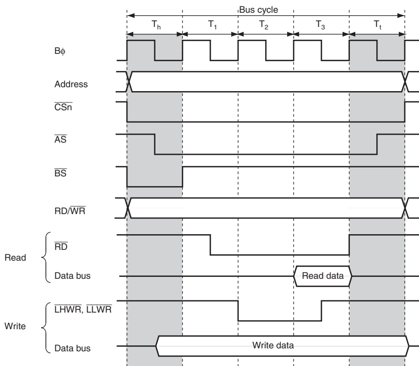
Figure 9.3 \overline{CS} and Address Assertion Period Extension (Example of Basic Bus Interface, 3-State Access Space, and RDNn = 0 )
