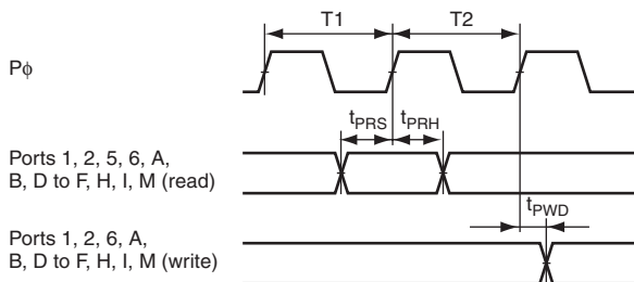
Figure 29.26 I/O Port Input/Output Timing
