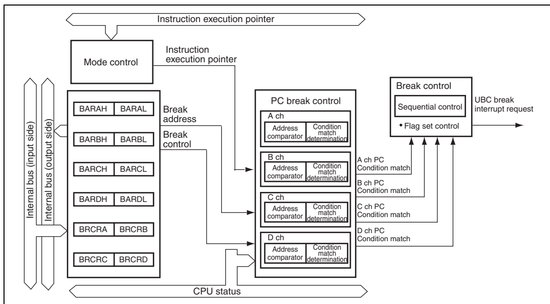
Figure 8.1 Block Diagram of UBC
