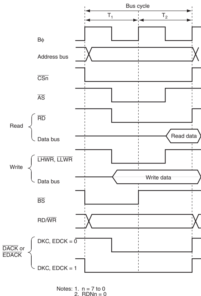
Figure 9.23 \overline{\text{DACK}} and \overline{\text{EDACK}} Signal Output Timings
