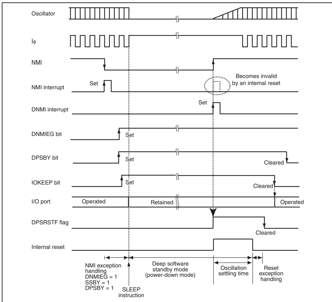
Figure 27.4 Deep Software Standby Mode Application Example (IOKEEP = 1)
