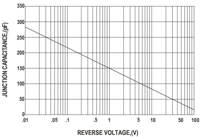
FIG.4-TYPICAL JUNCTION CAPACITANCE
