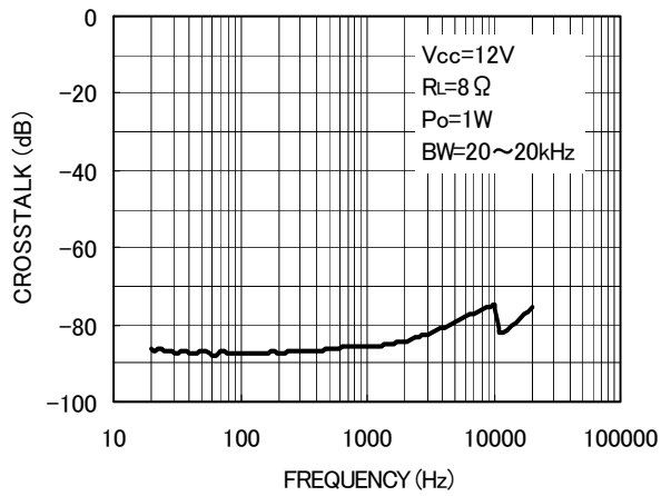
Fig. 4 Crosstalk - Frequency
