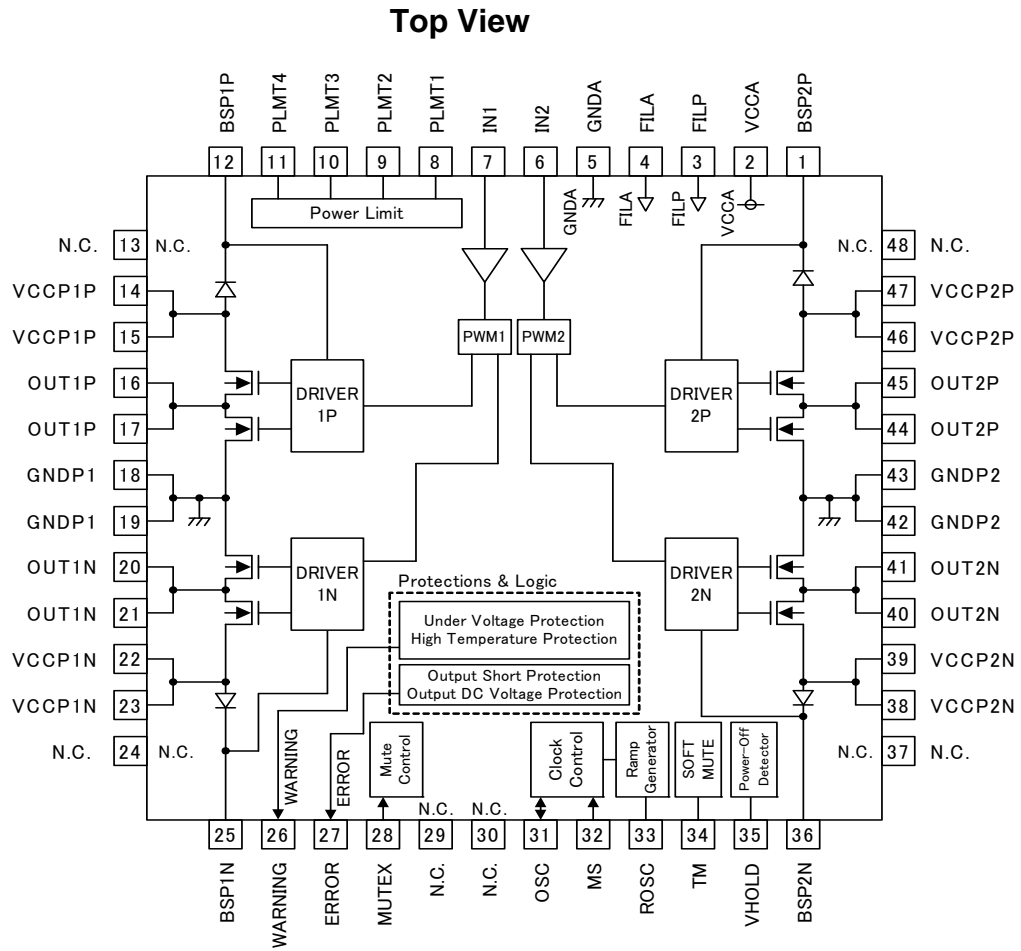
Fig. 23 Pin Assignment Diagram
