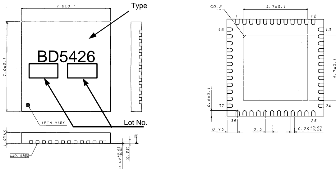
Fig. 24 Outer Dimensions and Inscriptions of VQFN048V7070 Package
