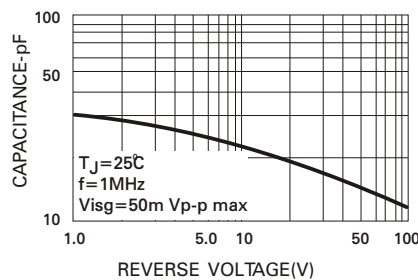
Fig.5 - TYPICAL JUNCTION CAPACITANCE
