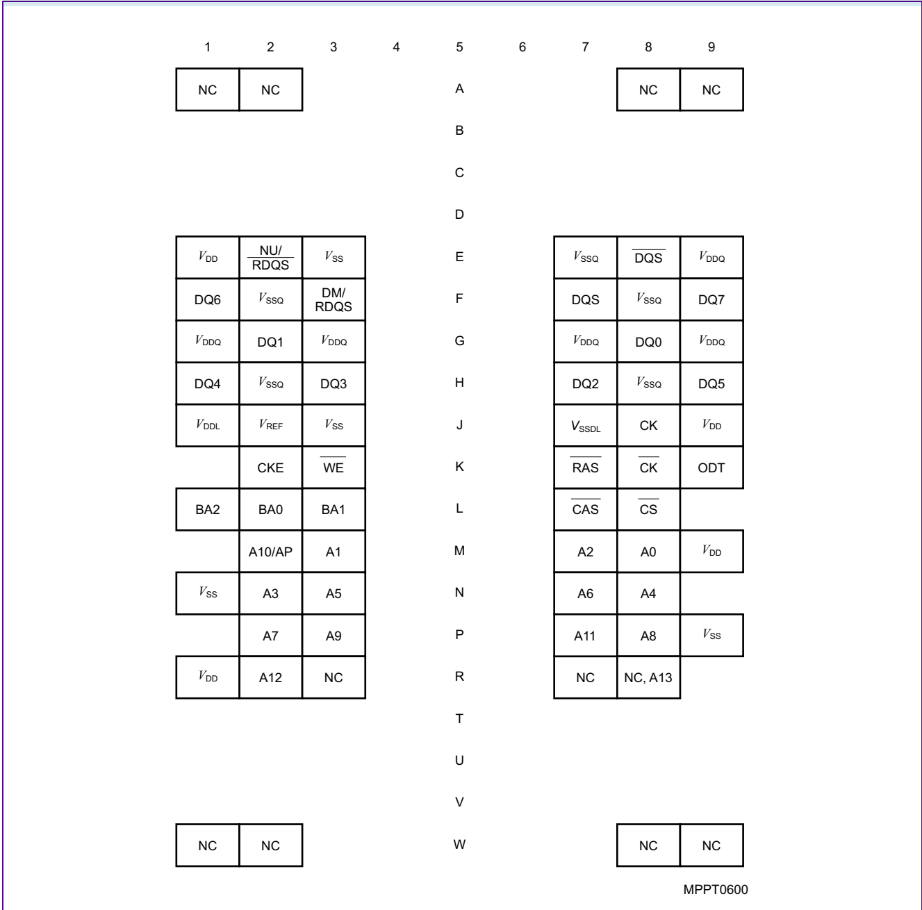
Ball Configuration for ×8 components, PG-TFBGA-68 (top view)
