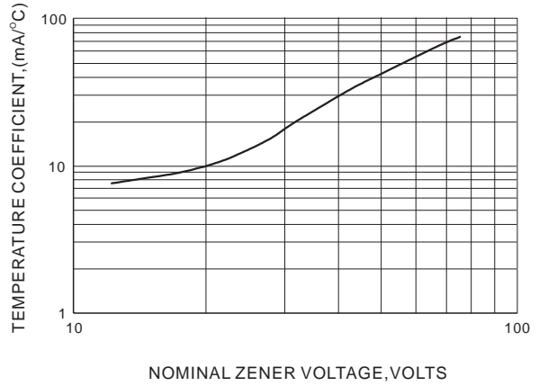
Fig.4 TEMPERATURE COEFFICIENTS
