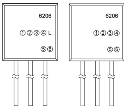
TO-92 (L Type) (SIDE VIEW)
