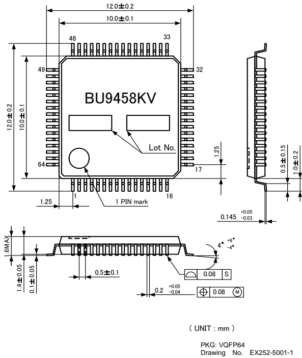
Figure 1. External dimension
