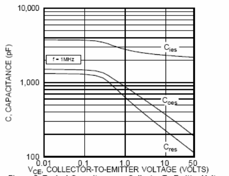
Figure 5, Typical Capacitance vs Collector-To-Emitter Voltage
