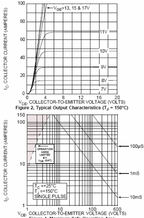
Figure 4, Maximum Safe Operating Area
