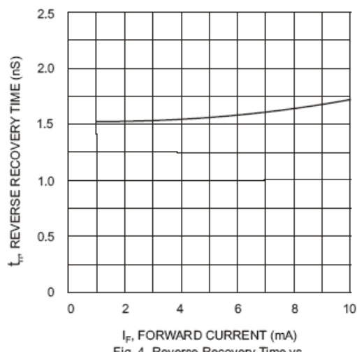
Fig. 4 Reverse Recovery Time vs. Forward Current
