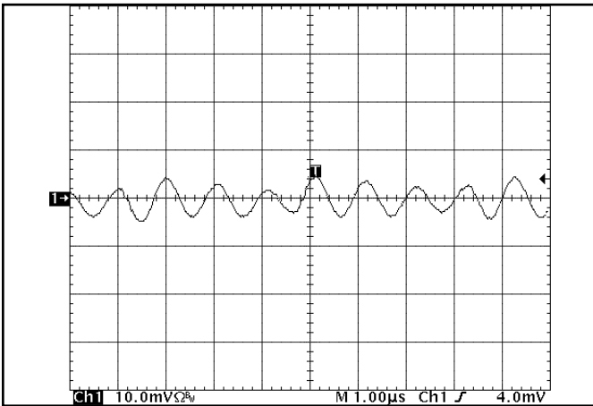
Figure 25: Input reflected ripple current, i_s , through a 10 \mu\text{H} source inductor at nominal input voltage and rated load current (5 mA/div). 1.225V and 2.45V outputs at 50% rated load current. (see Fig. 23)
